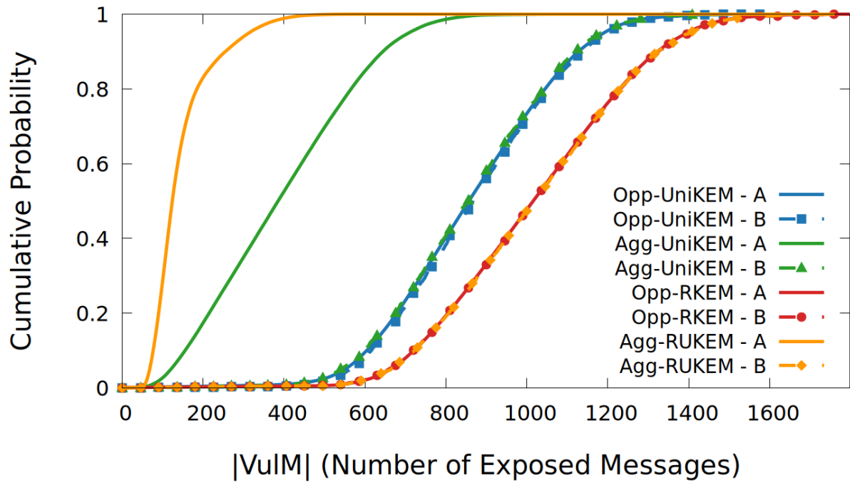
Vulnerable Message Set Size - CDF Comparison (Ratio traffic, Alice:Bob = 15:1)
