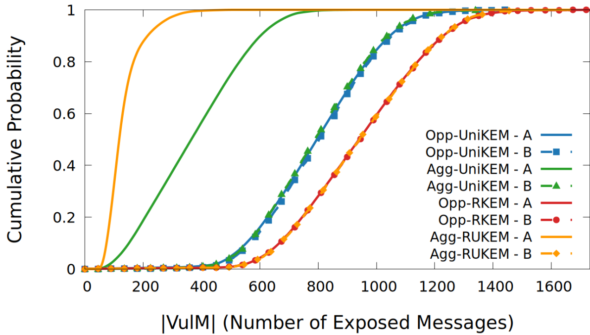
Vulnerable Message Set Size - CDF Comparison (Ratio traffic, Alice:Bob = 14:1)
