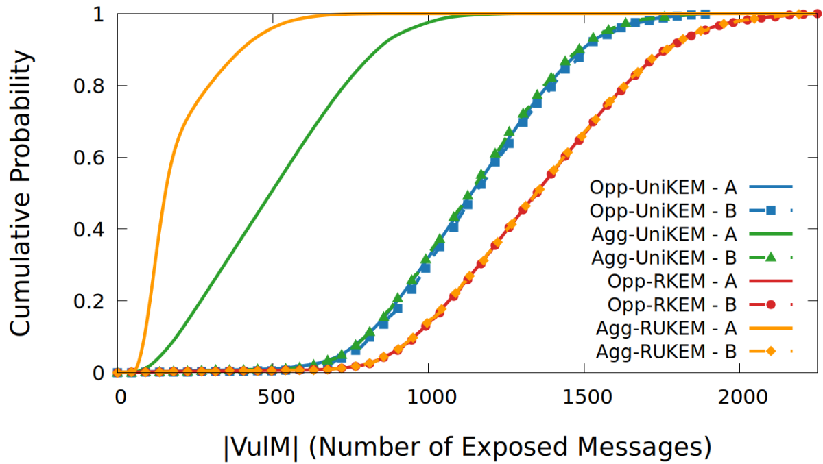
Vulnerable Message Set Size - CDF Comparison (Ratio traffic, Alice:Bob = 20:1)
