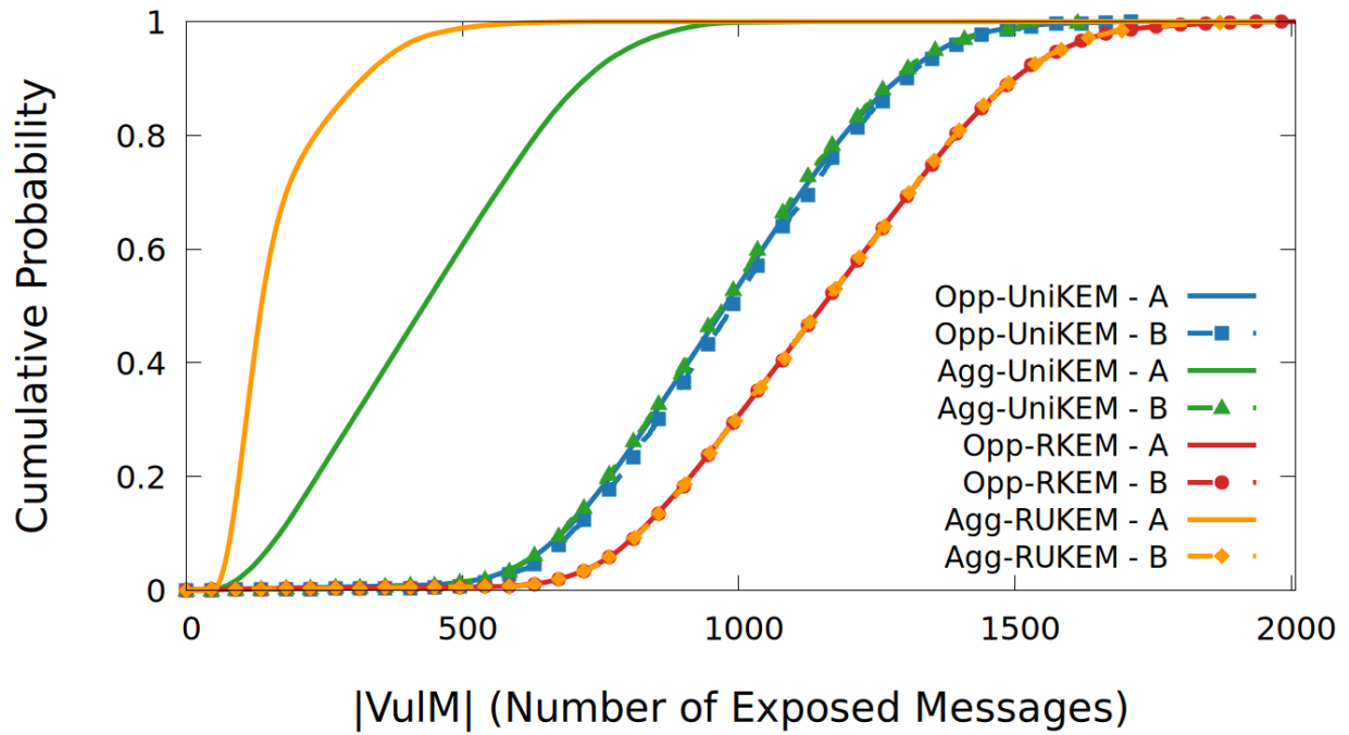
Vulnerable Message Set Size - CDF Comparison (Ratio traffic, Alice:Bob = 17:1)
