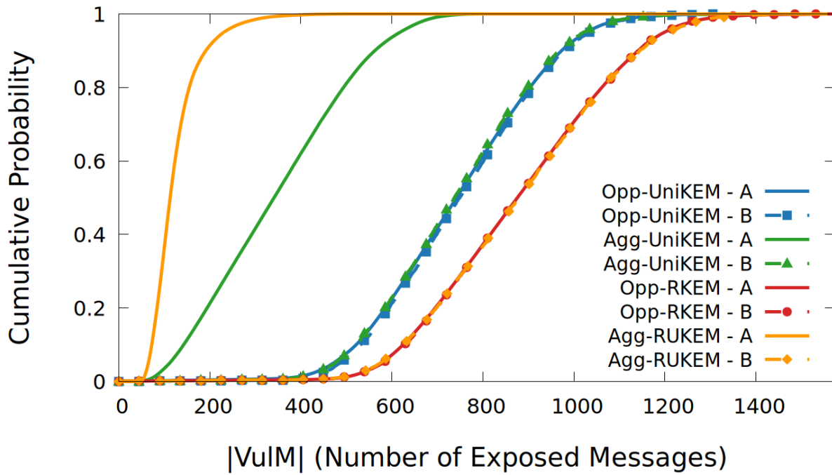
Vulnerable Message Set Size - CDF Comparison (Ratio traffic, Alice:Bob = 13:1)
