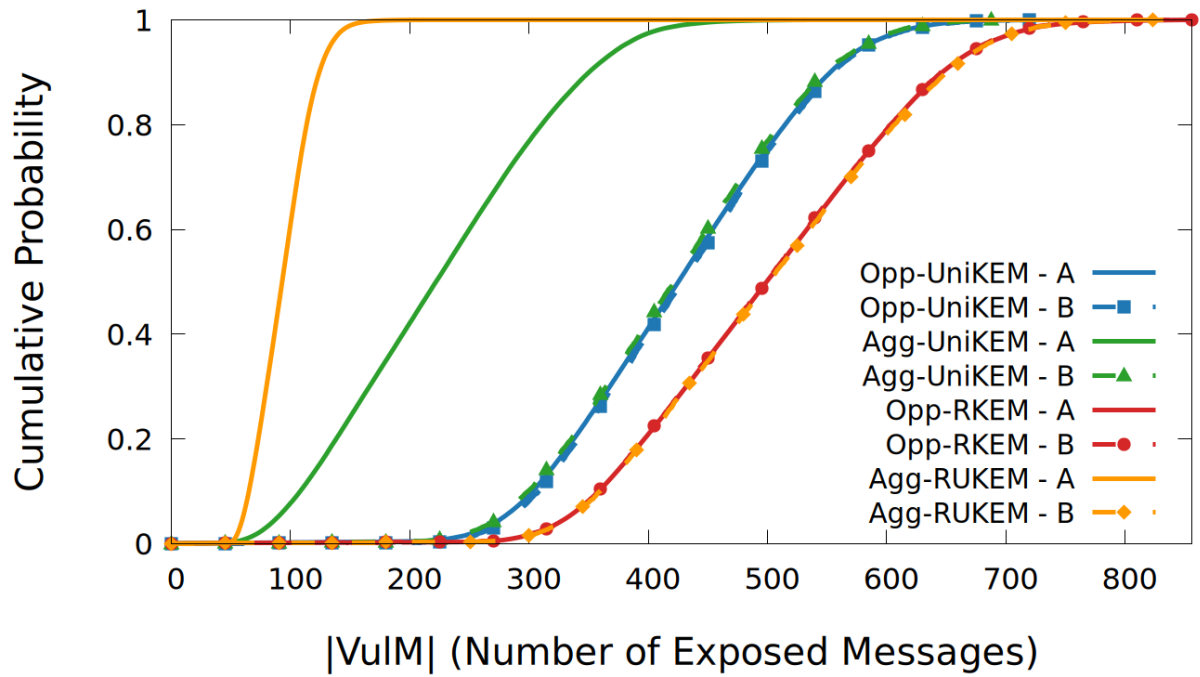
Vulnerable Message Set Size - CDF Comparison (Ratio traffic, Alice:Bob = 7:1)
