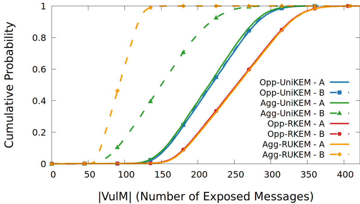
Vulnerable Message Set Size - CDF Comparison (Ratio traffic, Alice:Bob = 0.33:1)
