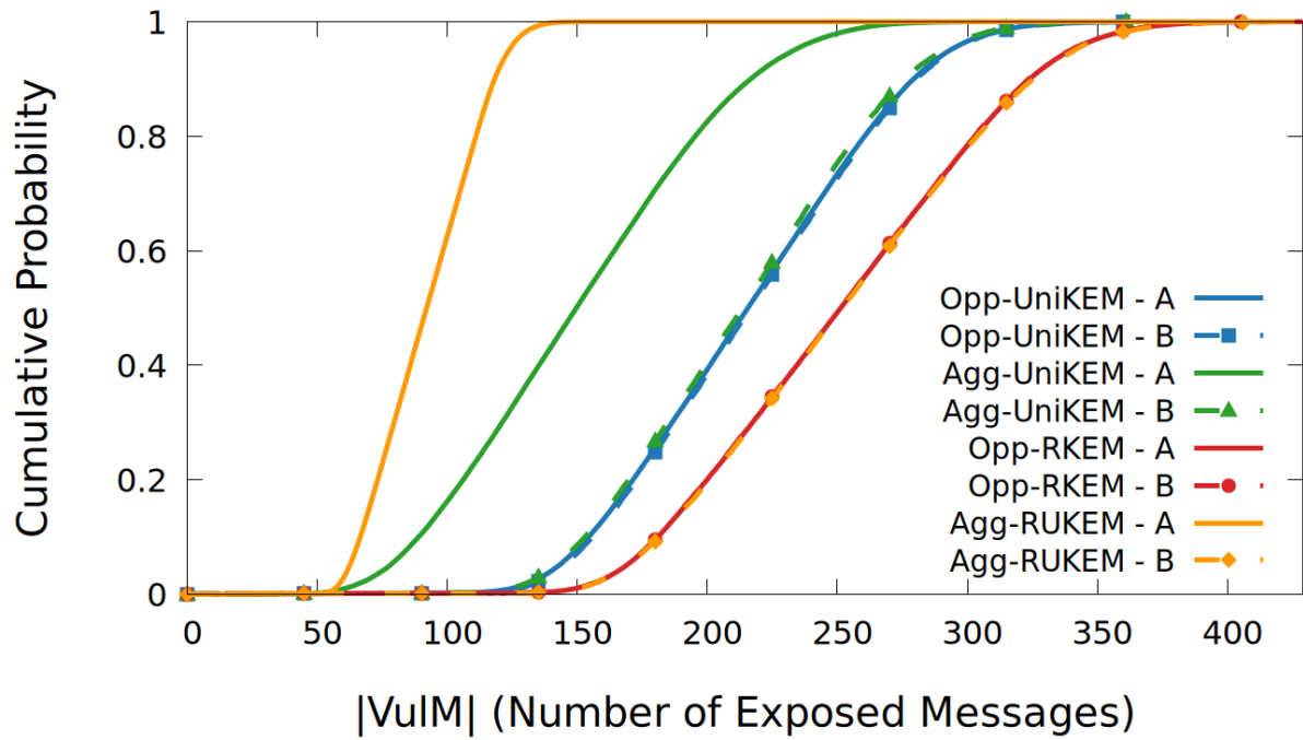
Vulnerable Message Set Size - CDF Comparison (Ratio traffic, Alice:Bob = 3:1)
