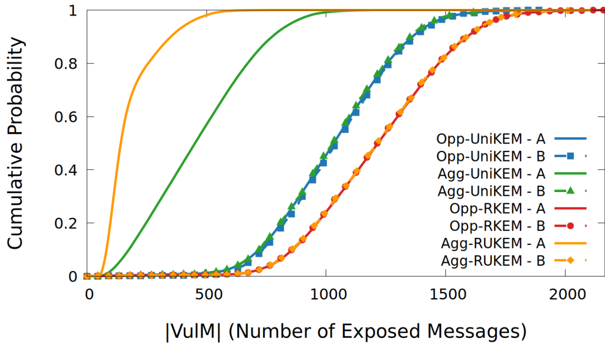
Vulnerable Message Set Size - CDF Comparison (Ratio traffic, Alice:Bob = 18:1)
