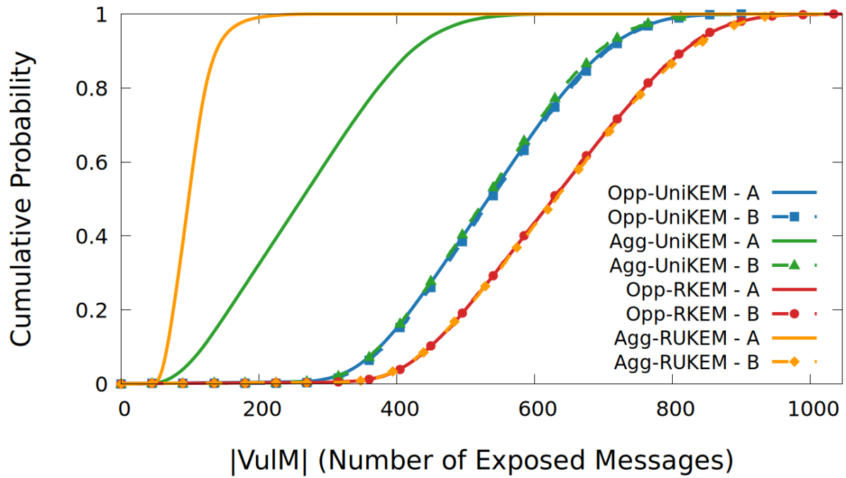
Vulnerable Message Set Size - CDF Comparison (Ratio traffic, Alice:Bob = 9:1)
