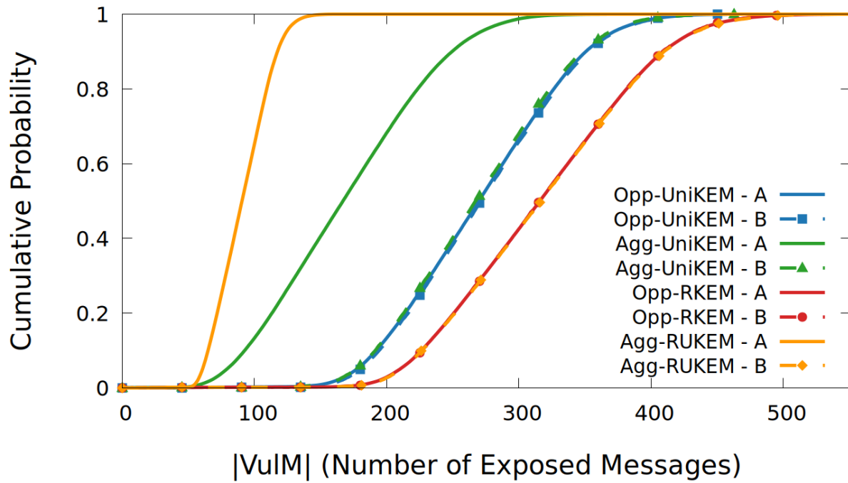
Vulnerable Message Set Size - CDF Comparison (Ratio traffic, Alice:Bob = 4:1)
