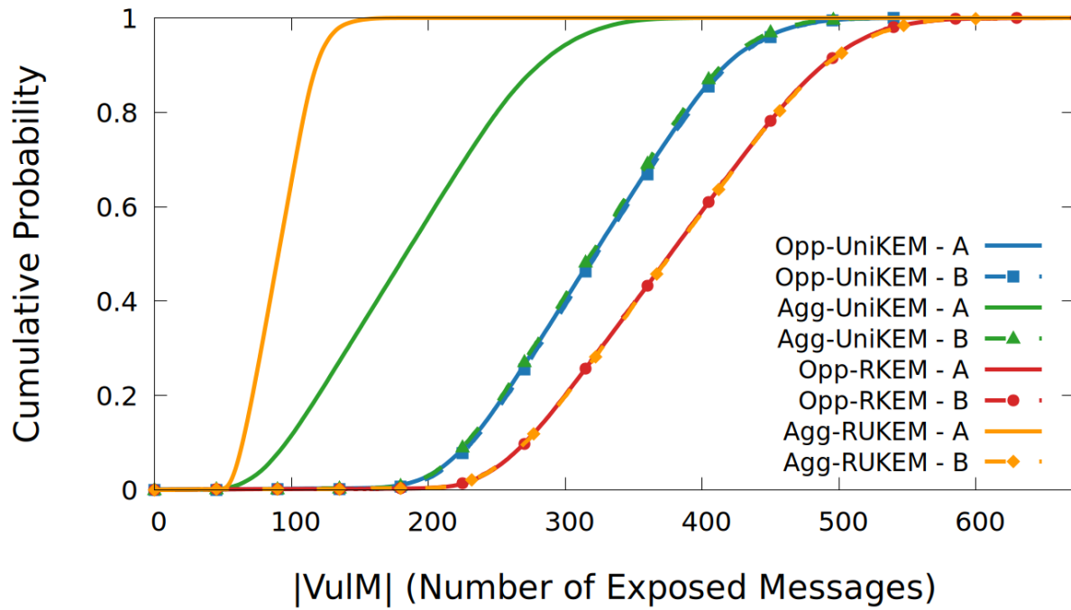
Vulnerable Message Set Size - CDF Comparison (Ratio traffic, Alice:Bob = 5:1)
