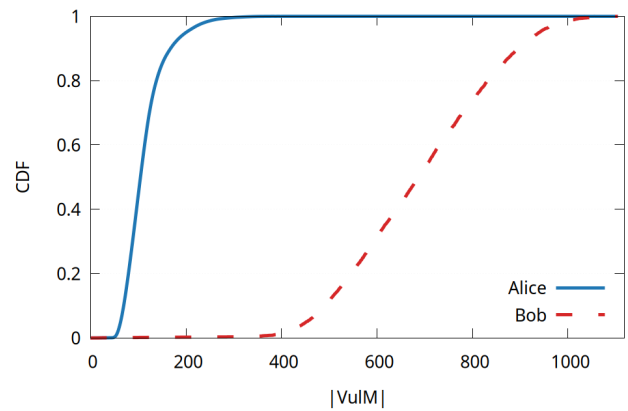
Agg-RUKEM, Alice:Bob = 10:1
