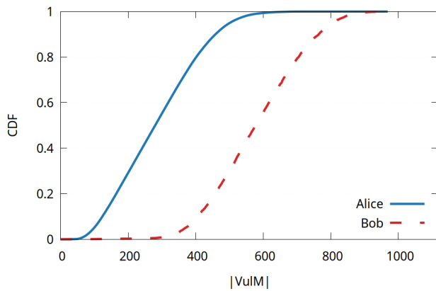
Agg-UniKEM, Alice:Bob = 10:1
