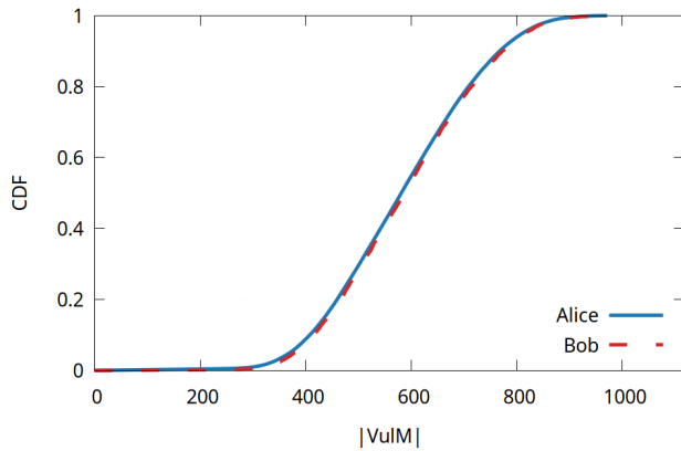
Opp-UniKEM, Alice:Bob = 10:1
