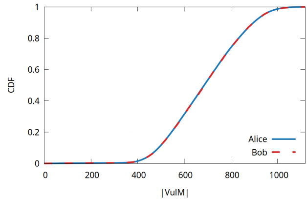
Opp-RKEM, Alice:Bob = 10:1
