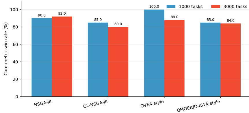
Fig. 7. ADARE core-metric win rate in the 20-repeat large-scale confirmatory protocol.
