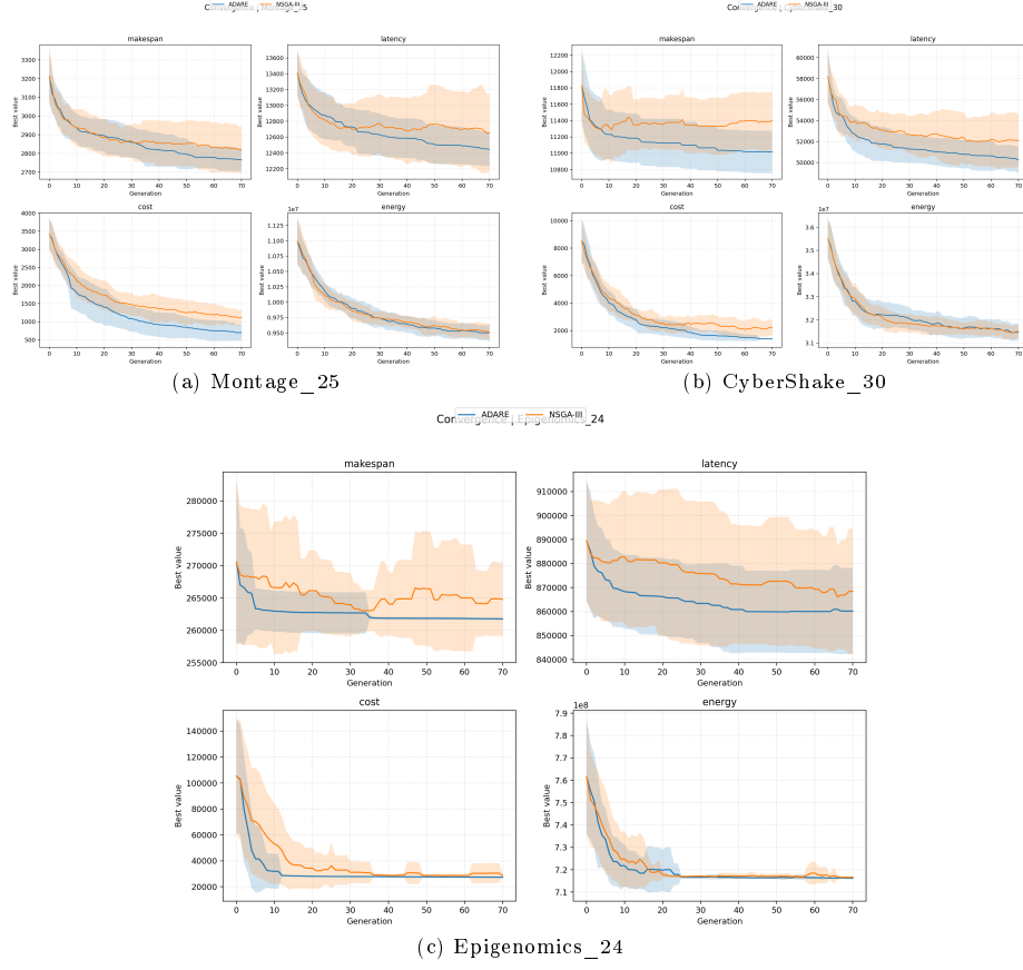
Fig. 10. Convergence traces (best objective values by generation) for Montage, CyberShake, and Epigenomics. Larger panels are used to improve readability of generation-wise trajectories and confidence bands.
