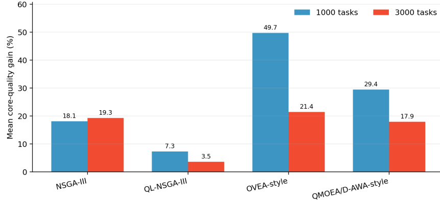
Fig. 6. Mean ADARE core-quality gain in the 20-repeat large-scale confirmatory protocol.
