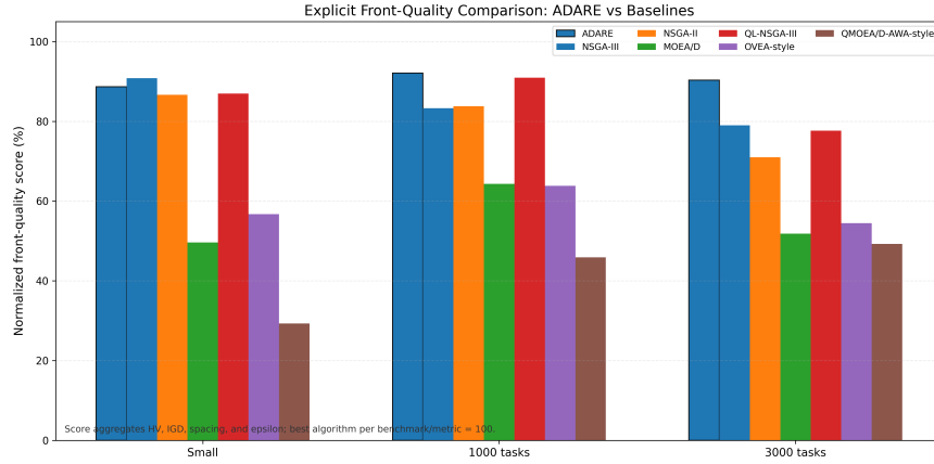
Fig. 5. Explicit normalized front-quality comparison between ADARE and all extended baselines.
