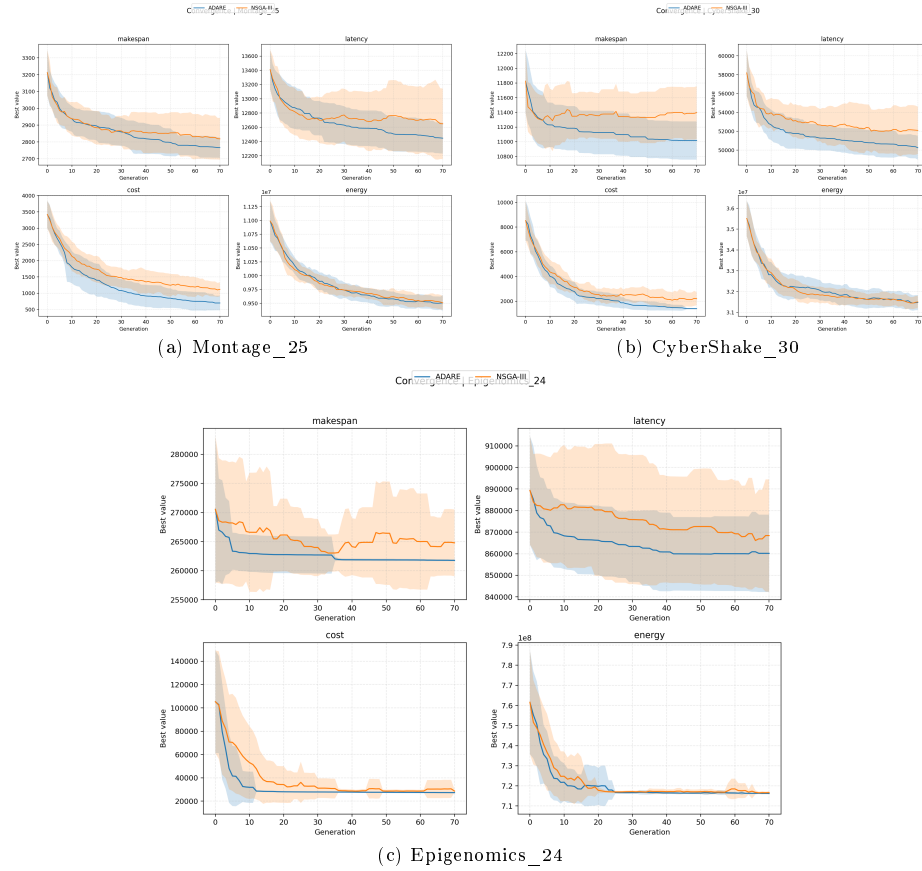
Fig. 8. Convergence traces (best objective values by generation) for Montage, CyberShake, and Epigenomics. Larger panels are used to improve readability of generation-wise trajectories and confidence bands.
