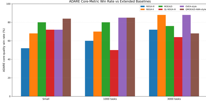
Fig. 4. ADARE core-metric win rate across scales and extended baselines.
