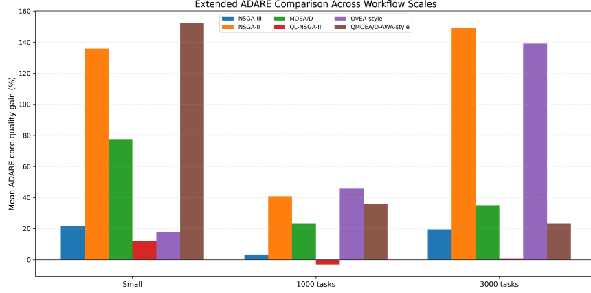
Fig. 3. Mean ADARE core-quality gain across scales and extended baselines.
