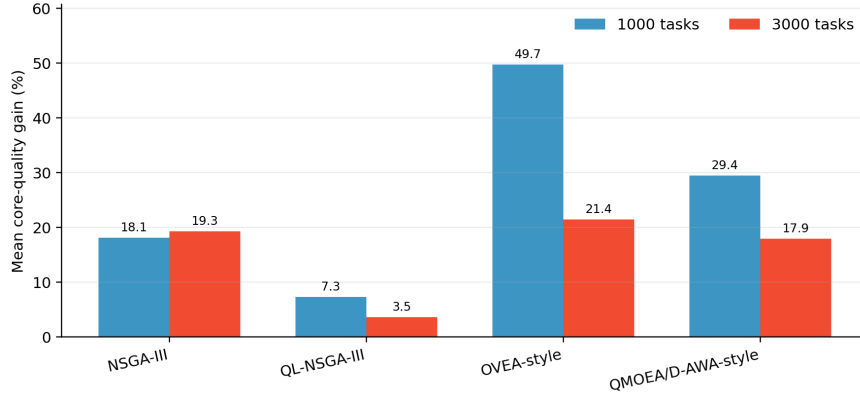
Fig. 5. Mean ADARE core-quality gain in the 20-repeat large-scale confirmatory protocol.
