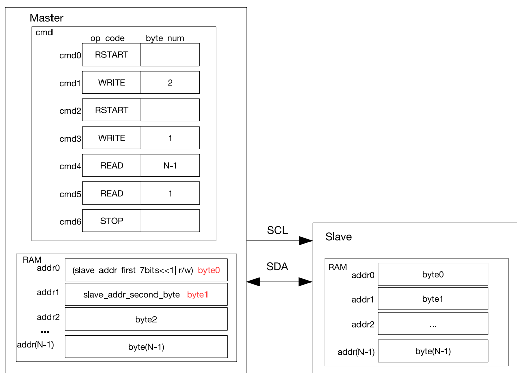
Figure 30.7-6. I2C master Reading I2C slave with a 10-bit Address
