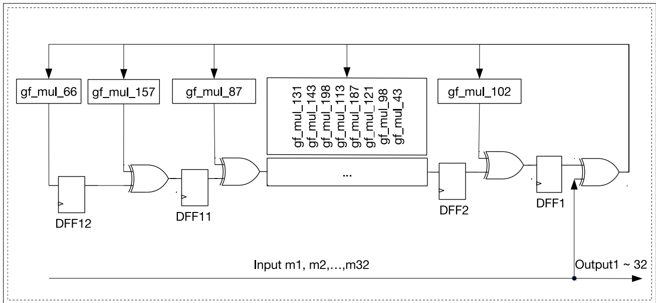
Figure 5.3-2. Shift Register Circuit (first 32 output)
