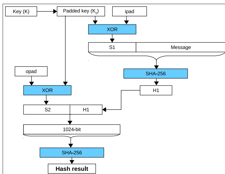
Figure 21.6-2. HMAC Structure Schematic Diagram
