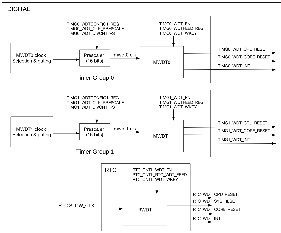
Figure 13.2-1. Digital Watchdog Timers in ESP32-C5
