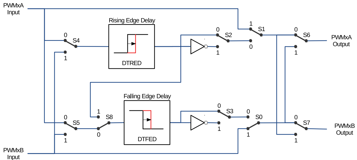
Figure 36.3-21. Options for Setting up the Dead Time Generator Module
