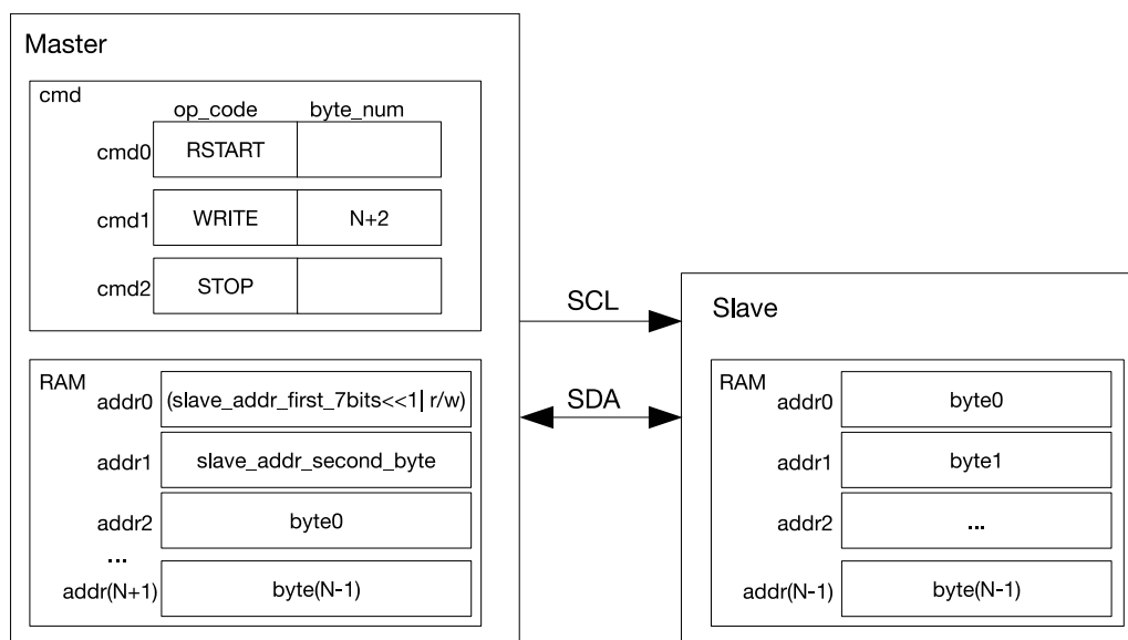
Figure 30.7-2. I2C master Writing to a Slave with a 10-bit Address
