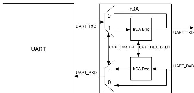
Figure 28.4-7. IrDA Encoding and Decoding Diagram
