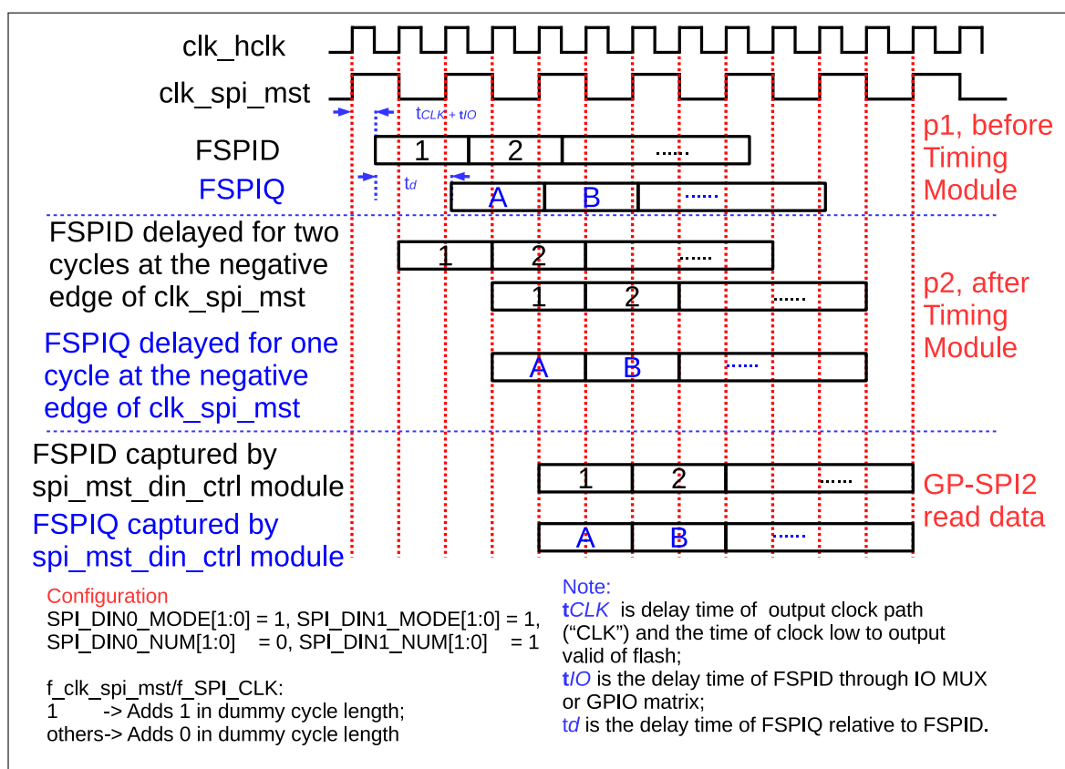
Figure 29.8-2. Timing Compensation Example in GP-SPI2
