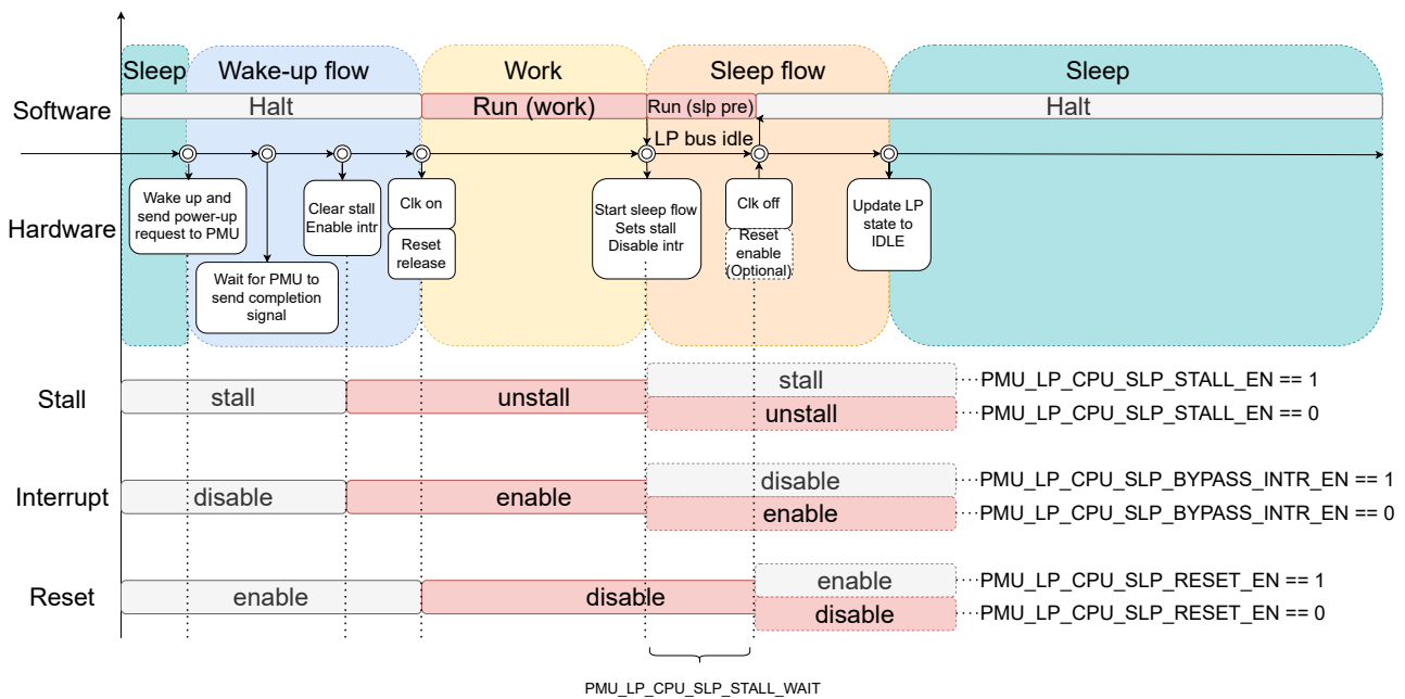
Figure 2.9-1. Wake-Up and Sleep Flow of LP CPU
