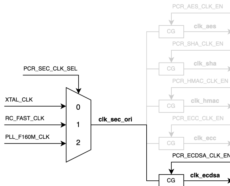
Figure 25.5-2. clk_ecdsa Diagram
