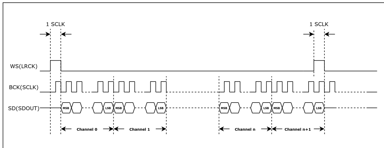
Figure 31.5-3. TDM PCM Standard Timing Diagram
