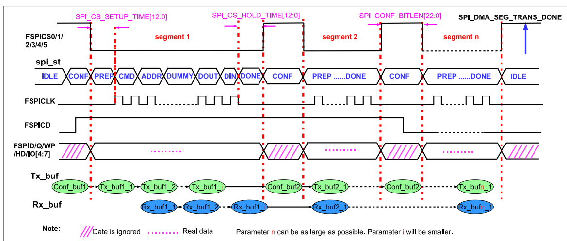
Figure 29.5-9. Configurable Segmented Transfer
