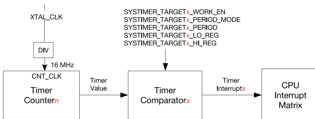
Figure 11.5-1. System Timer Alarm Generation
