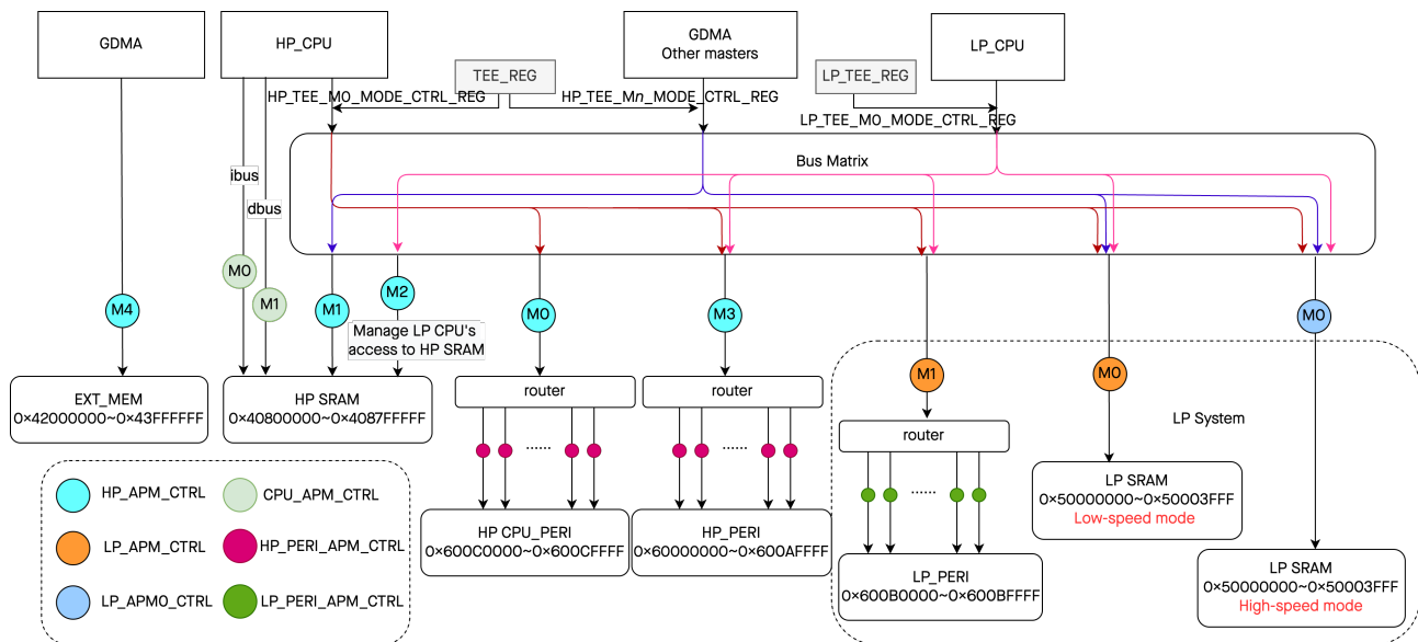
Figure 15.5-1. APM Controller Architecture
