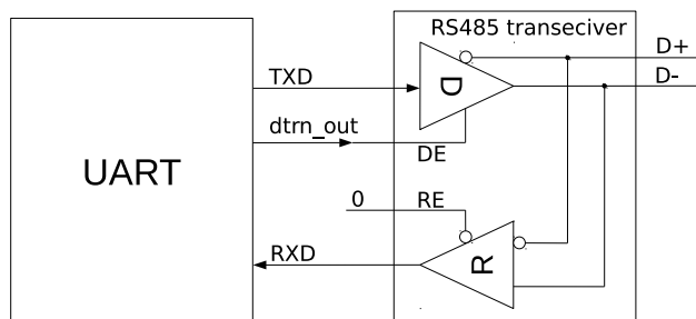
Figure 28.4-5. Driver Control Diagram in RS485 Mode
