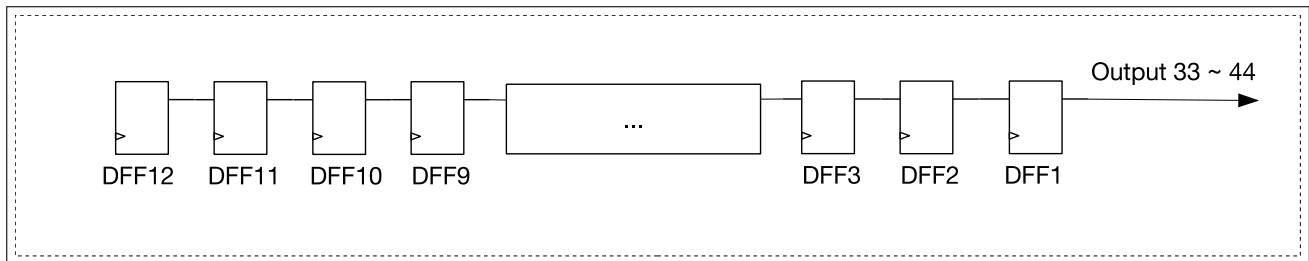
Figure 5.3-3. Shift Register Circuit (last 12 output)
