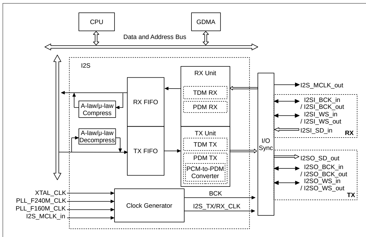
Figure 31.4-1. ESP32-C5 I2S System Diagram
