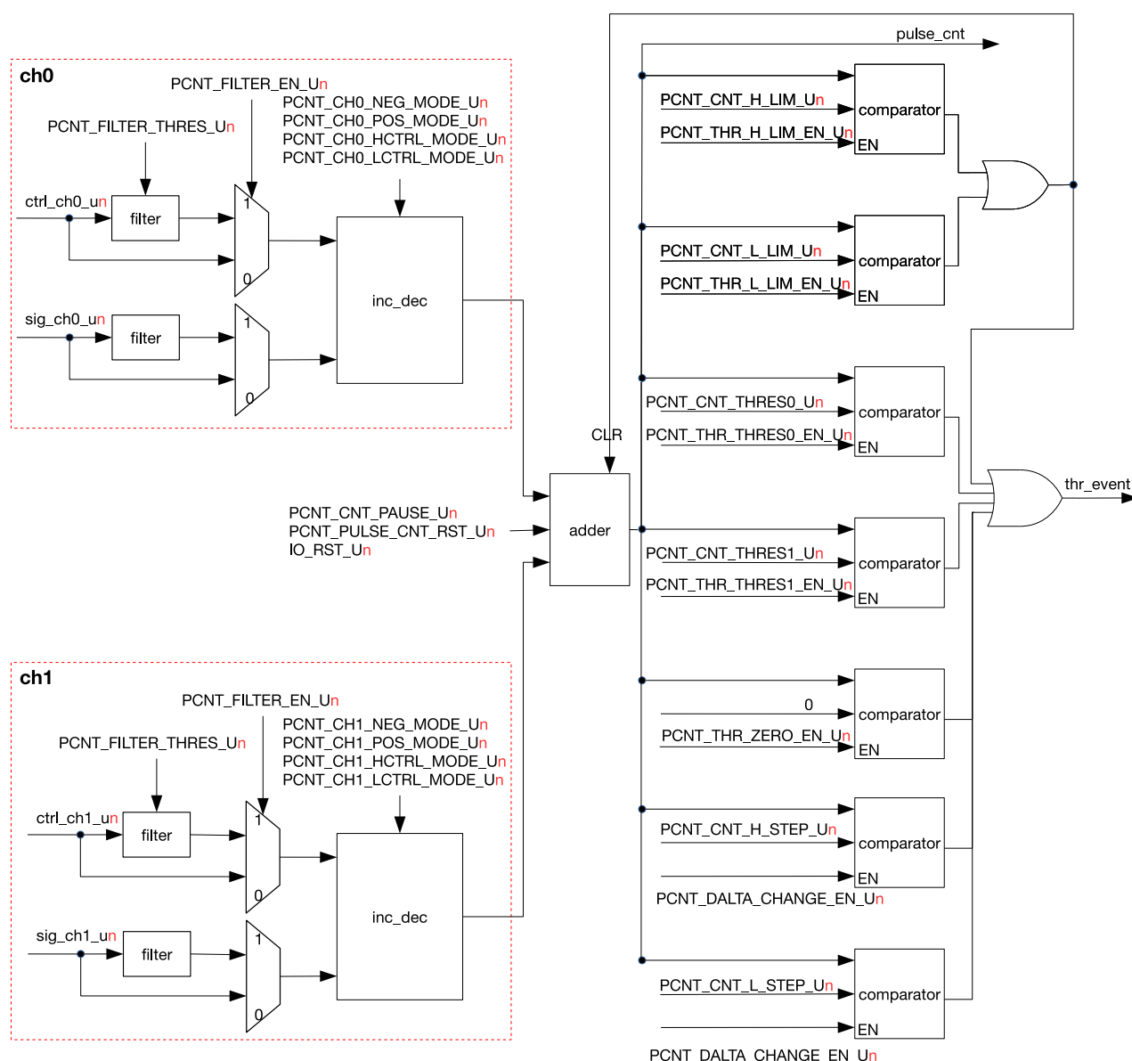
Figure 32.2-1. PCNT Unit Architecture
