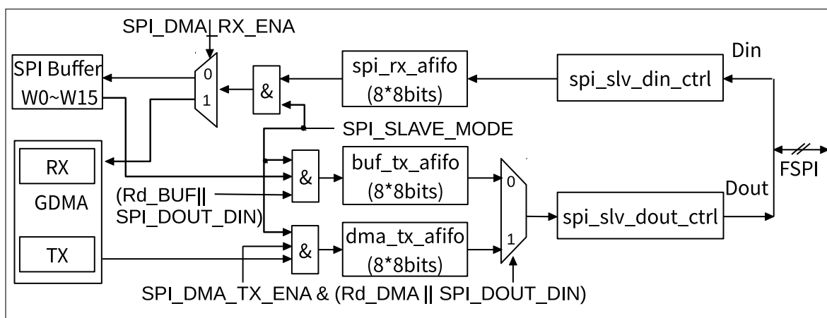
Figure 29.5-4. Data Flow Control When GP-SPI2 Works as Slave
