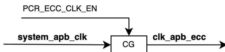
Figure 20.4-2. clk_apb_ecc Diagram
