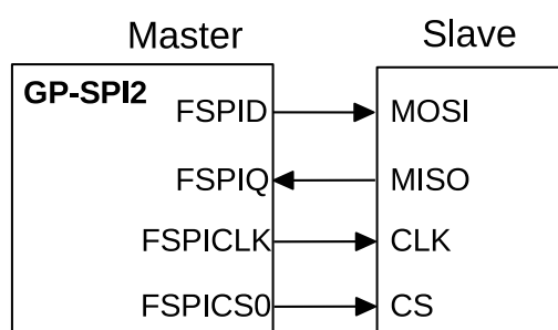
Figure 29.5-6. Full-Duplex Communication Between GP-SPI2 Master and a Slave
