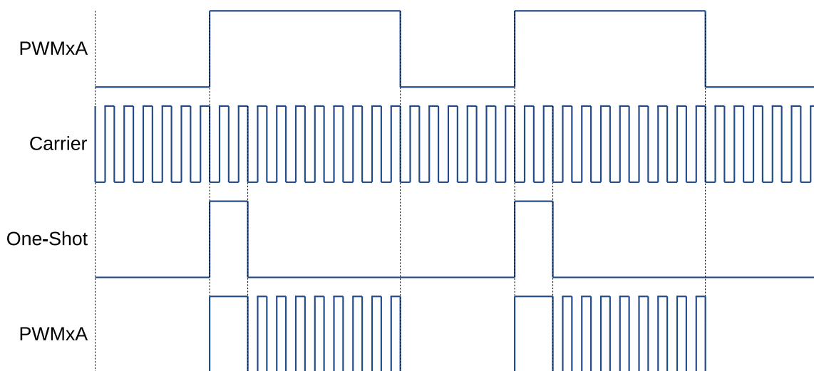
Figure 36.3-27. Example of the First Pulse and the Subsequent Sustaining Pulses of the PWM Carrier Submodule
