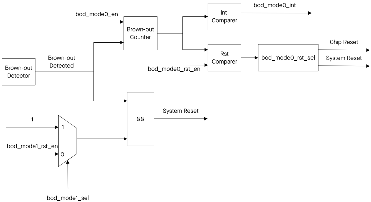
Figure 18.3-2. Brown-out Reset Workflow
