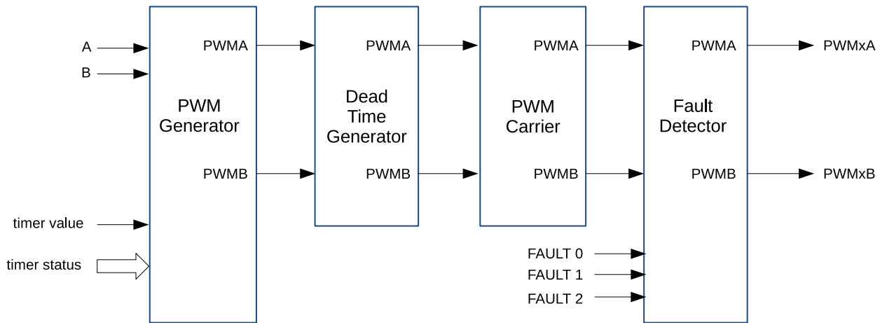
Figure 36.3-12. Block Diagram of A PWM Operator
