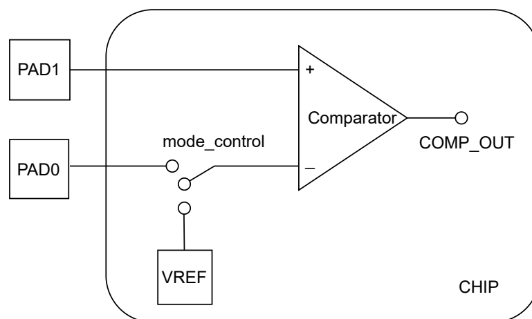
Figure 42.3-1. Analog Voltage Comparator Architecture
