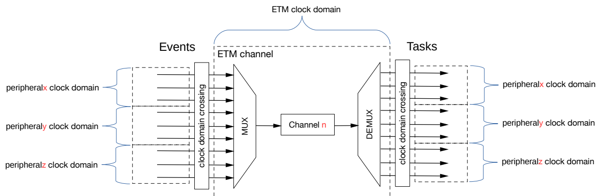
Figure 10.3-2. Event Task Matrix Clock Architecture
