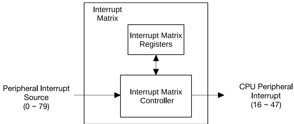
Figure 9.4-1. Interrupt Matrix Structure
