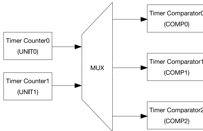
Figure 11.3-1. System Timer Structure
