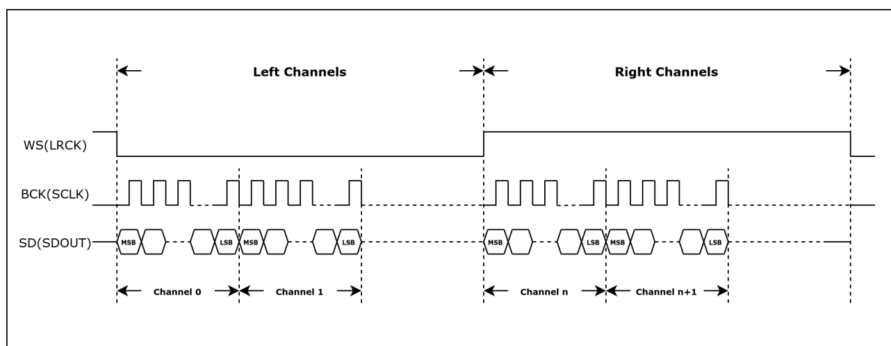
Figure 31.5-2. TDM MSB Alignment Standard Timing Diagram
