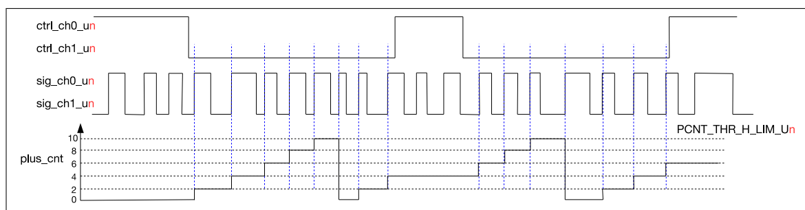
Figure 32.3-3. Two Channels Up Counting Diagram
