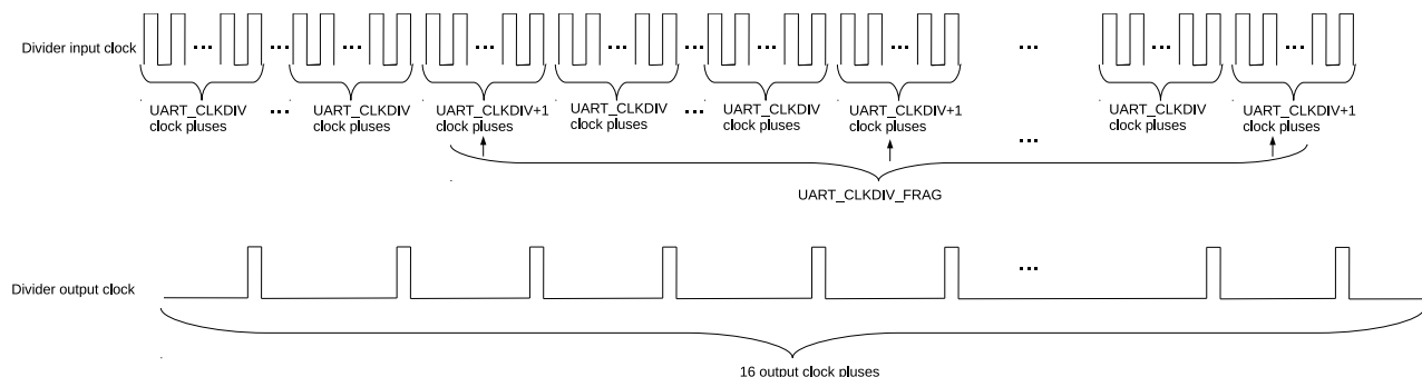
Figure 28.4-1. UART Controllers Division
