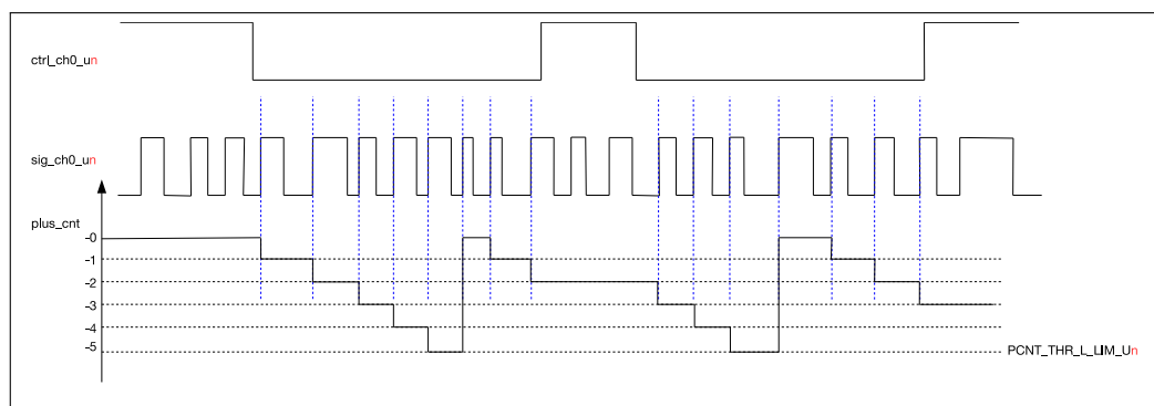
Figure 32.3-2. Channel 0 Down Counting Diagram
