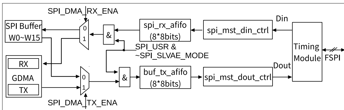
Figure 29.5-3. Data Flow Control When GP-SPI2 Works as Master
