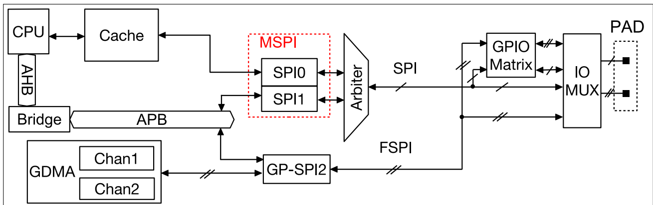
Figure 29.4-1. SPI Module Overview
