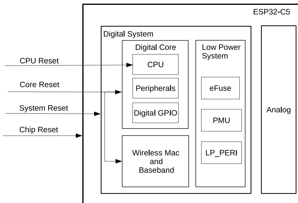
Figure 7.1-1. Reset Types
