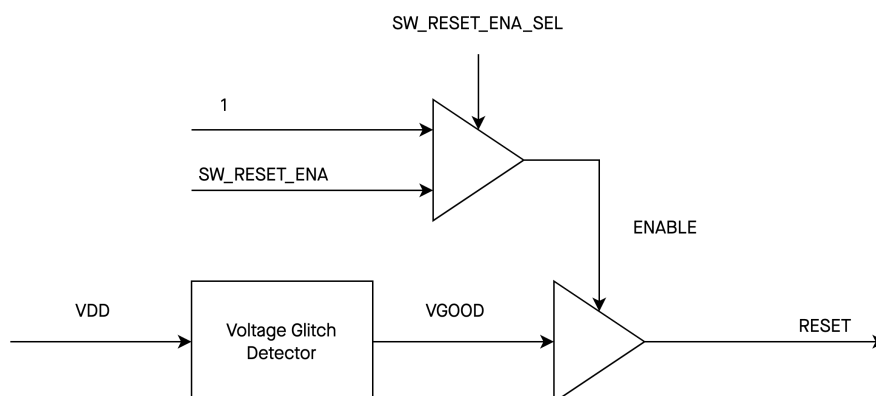
Figure 18.3-3. Structure of Voltage Glitch Detectors
