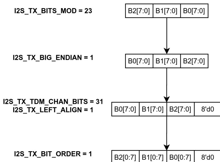
Figure 31.9-1. TX Data Format Control
