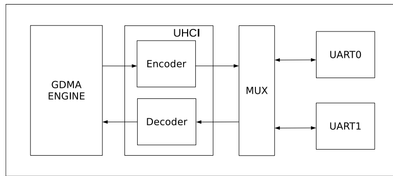
Figure 28.4-10. Data Transfer in GDMA Mode
