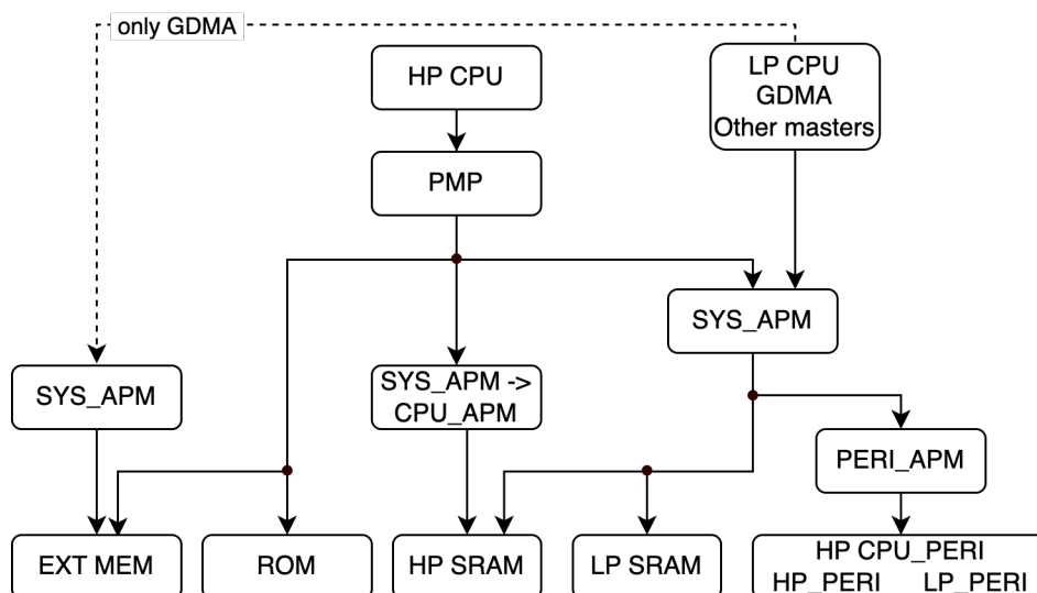
Figure 15.1-1. PMP-APM Management Relation
