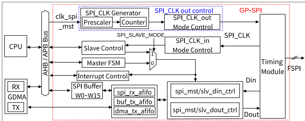
Figure 29.5-2. GP-SPI2 Functional Blocks
