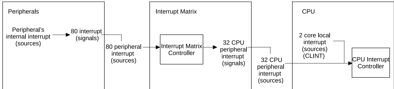
Figure 9.2-1. Interrupt Flow in ESP32-C5
