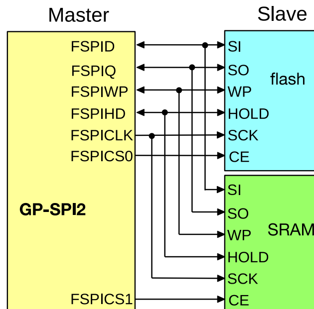
Figure 29.5-7. Connection of GP-SPI2 to Flash and External RAM in 4-bit Mode
