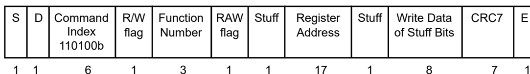
Figure 34.5-1. CMD52 Content
