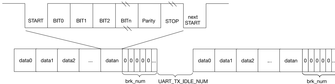
Figure 28.4-3. Structure of UART Data Frame
