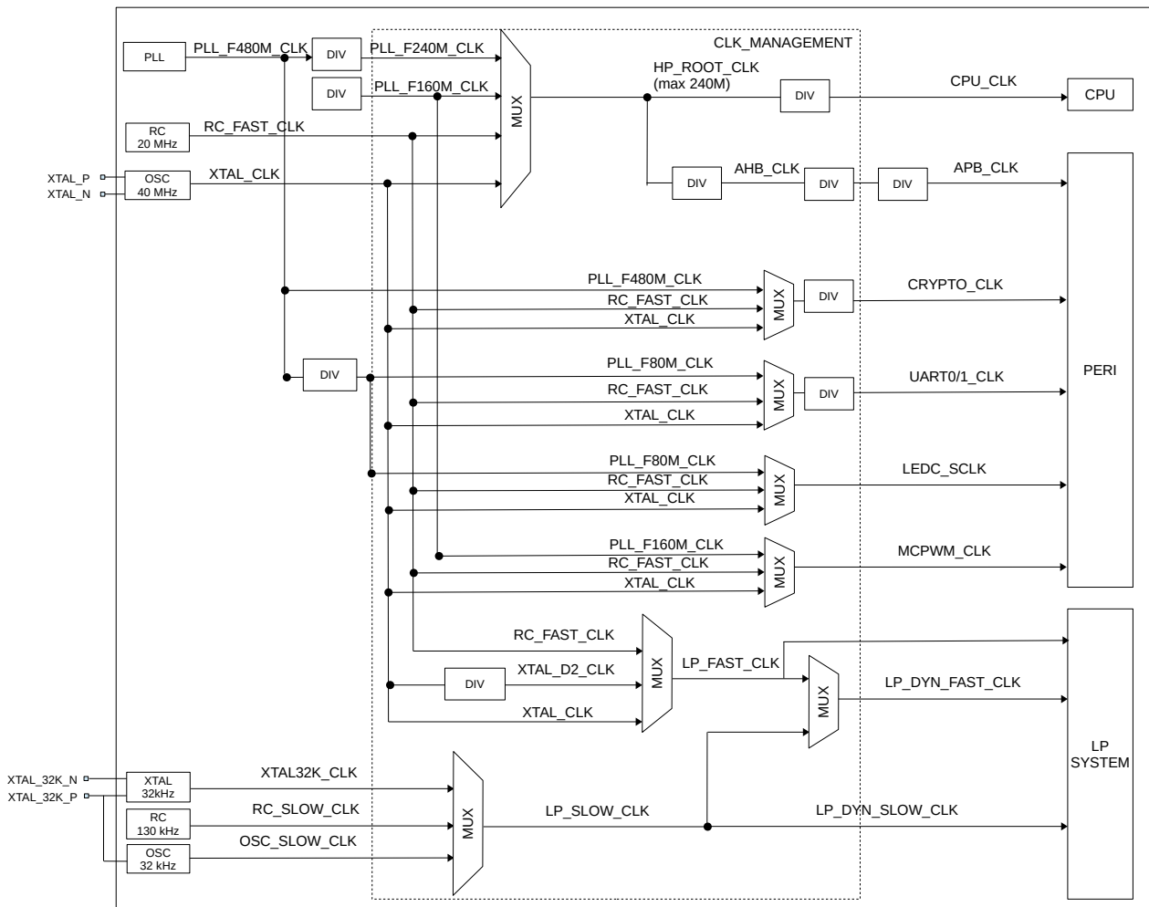
Figure 7.2-1. System Clock
