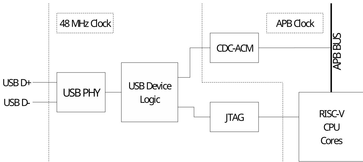
Figure 33.2-1. USB Serial/JTAG High Level Diagram
