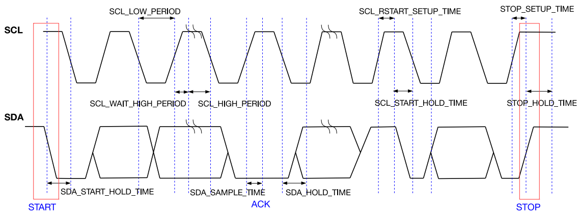
Figure 30.4-1. I2C Timing Diagram
