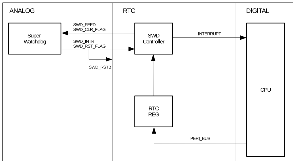
Figure 13.3-1. Super Watchdog Controller Structure
