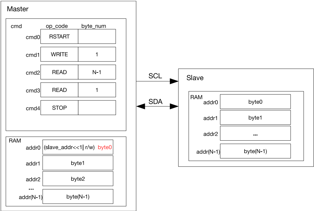
Figure 30.7-5. I2C master Reading I2C slave with a 7-bit Address
