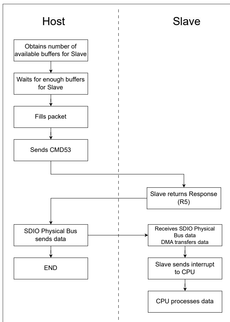
Figure 34.7-2. Procedure of Slave Receiving Packets from Host
