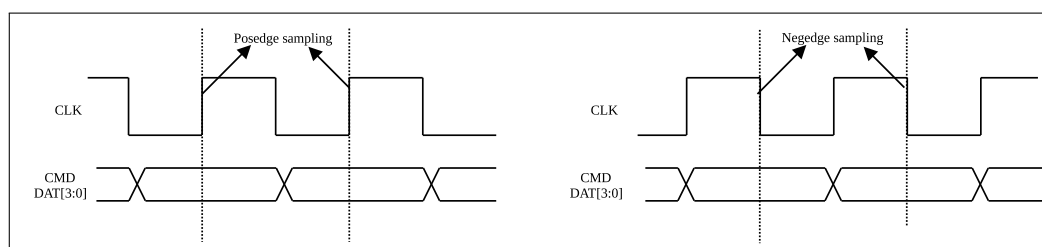
Figure 34.5-8. Sampling Timing Diagram
