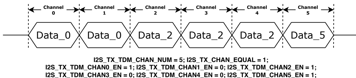
Figure 31.9-2. TDM Channel Control
