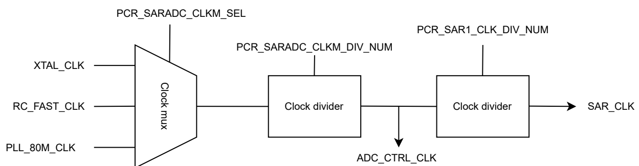
Figure 41.5-1. SAR ADC Clock Structure
