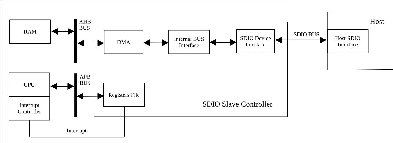
Figure 34.3-1. SDIO Slave Block Diagram
