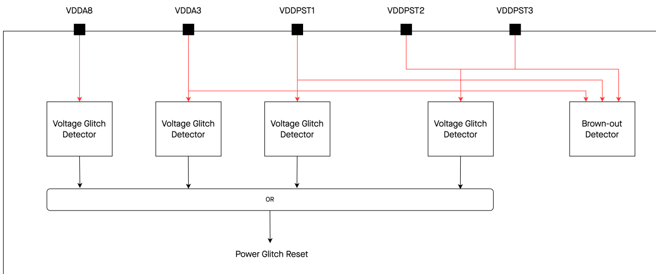
Figure 18.3-1. Architecture of Power Supply Detector
