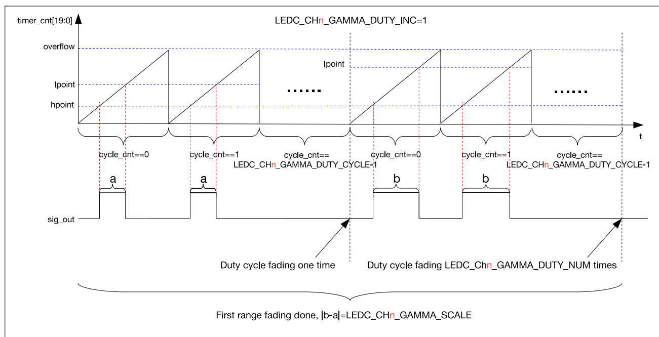
Figure 35.4-4. Output Signal of Linear Duty Cycle Fading
