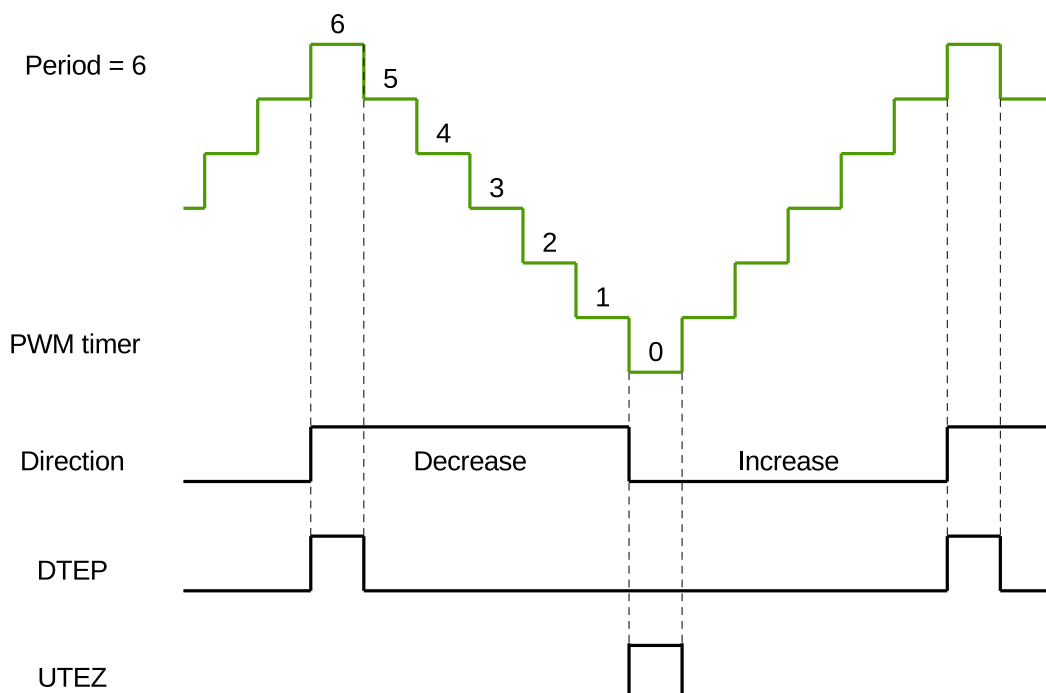
Figure 36.3-11. DTEP and UTEZ Generation in Count-Up-Down Mode
