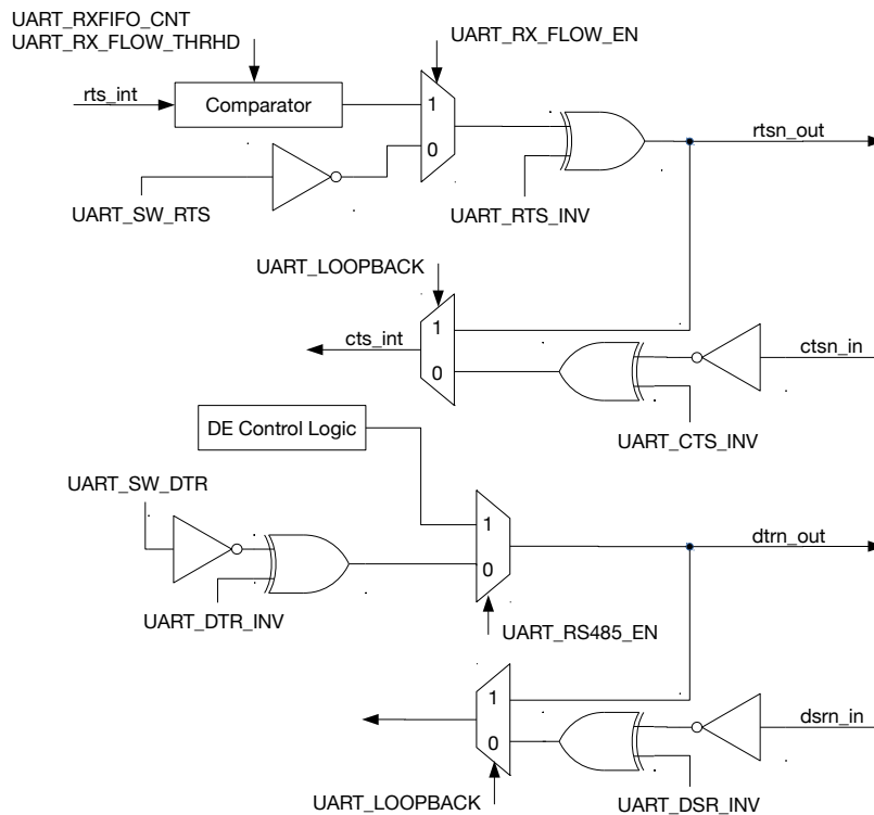
Figure 28.4-8. Hardware Flow Control Diagram
