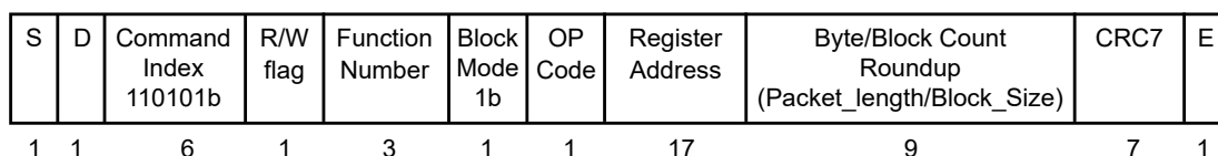
Figure 34.5-2. CMD53 Content
