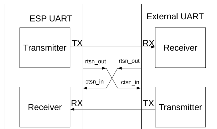
Figure 28.4-9. Connection between Hardware Flow Control Signals
