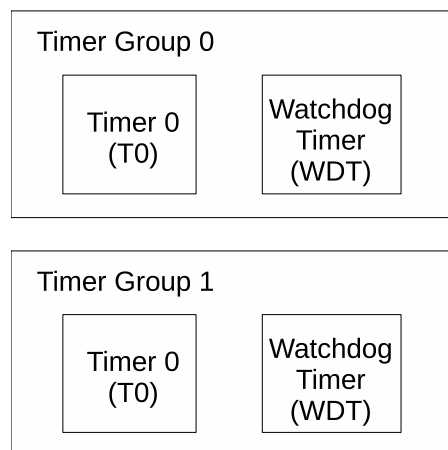
Figure 12.1-1. Timer Group Overview
