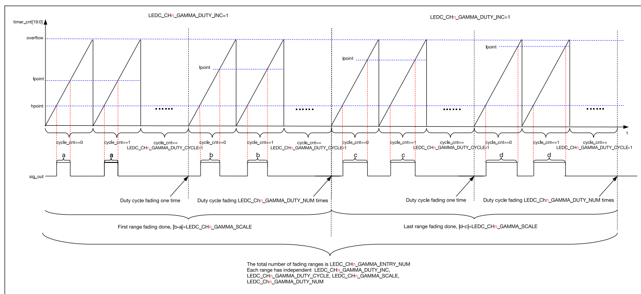
Figure 35.4-5. Output Signal of Gamma Curve Fading
