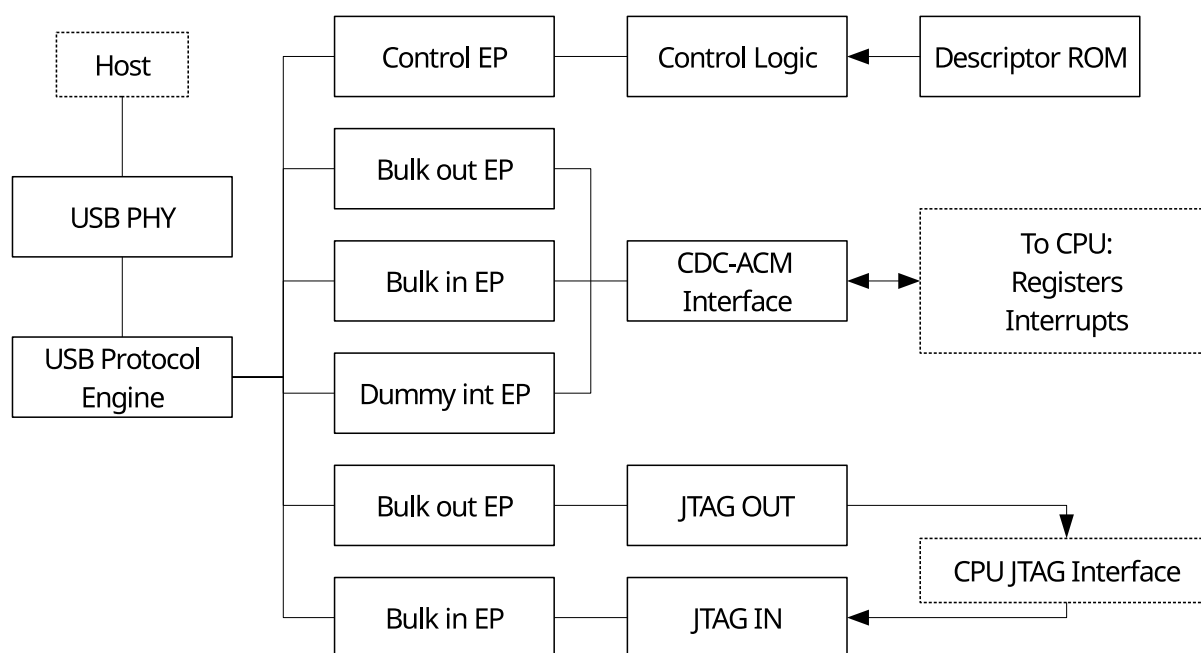
Figure 33.2-2. USB Serial/JTAG Block Diagram
