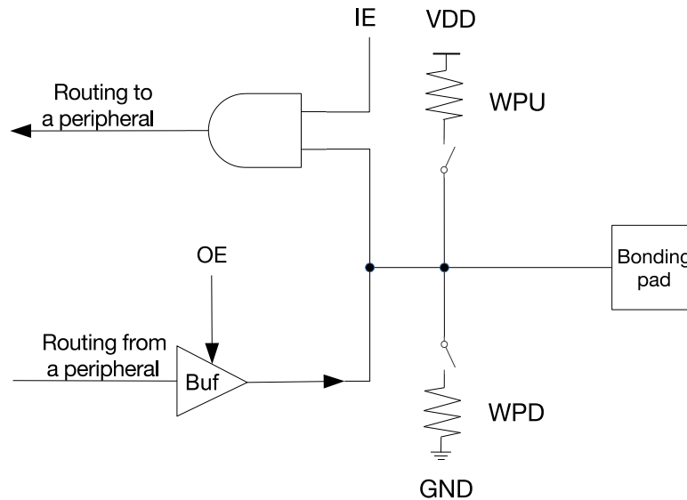
Figure 6.3-2. Internal Structure of a Pad
