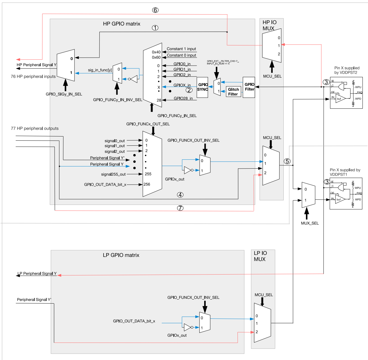
Figure 6.3-1. Architecture of HP GPIO Matrix, HP IO MUX, LP GPIO Matrix, and LP IO MUX
