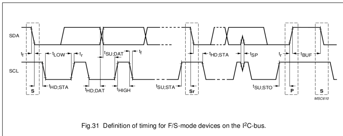
Figure 30.3-3. I2C Protocol Timing (Cited from Fig.31 in The I2C-bus specification Version 2.1)
