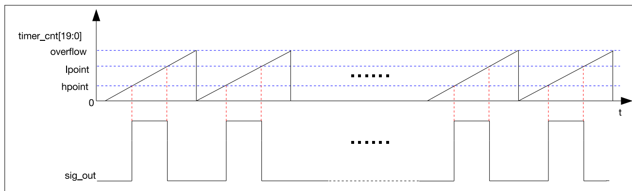
Figure 35.4-3. LED PWM Output Signal Diagram
