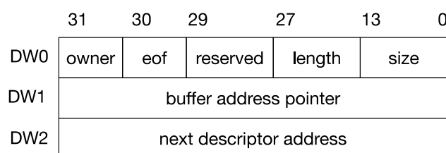
Figure 34.5-5. DMA Linked List Descriptor Structure of the SDIO Slave
