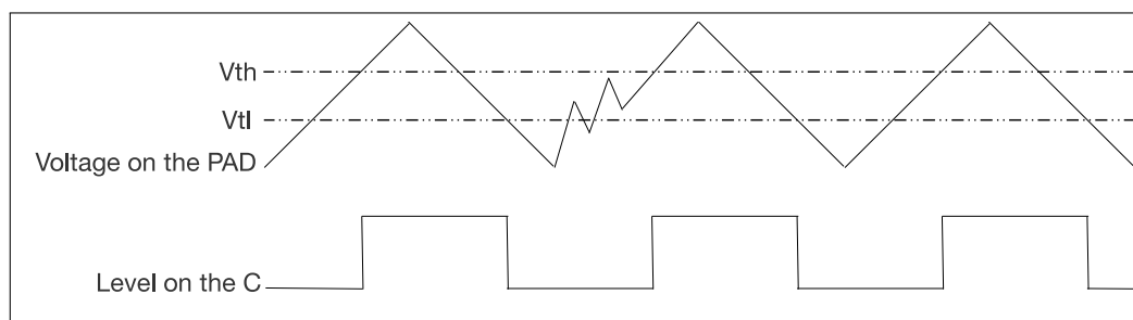
Figure 6.10-2. Example of Level Flip on the Chip Pad — Hysteresis Function Enabled
