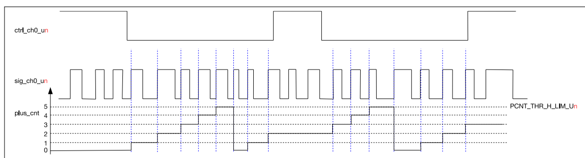
Figure 32.3-1. Channel 0 Up Counting Diagram
