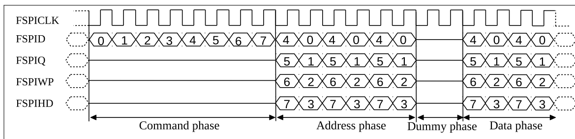
Figure 29.5-8. SPI Quad I/O Read Command Sequence Sent by GP-SPI2 to Flash
