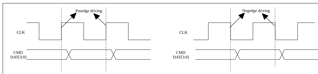
Figure 34.5-9. Output Timing Diagram
