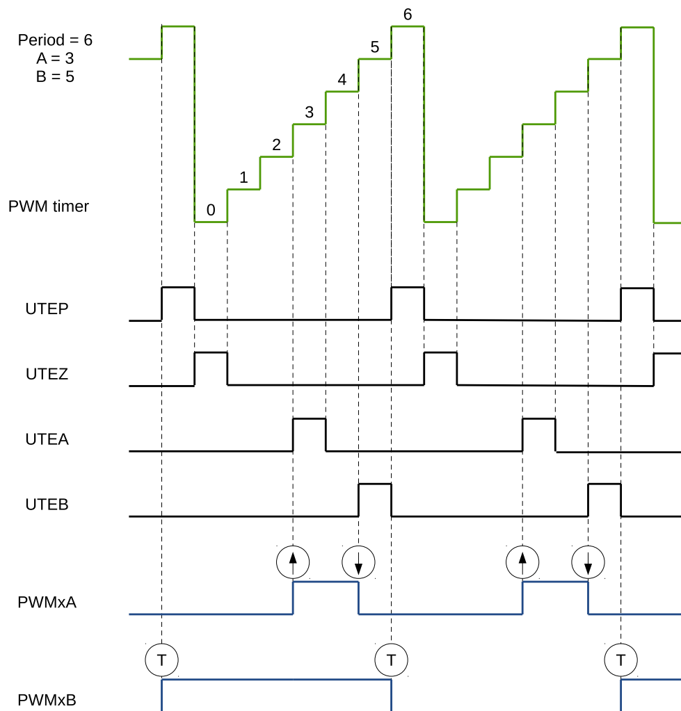
Figure 36.3-15. Count-Up, Pulse Placement Asymmetric Waveform with Independent Modulation on PWMxA
