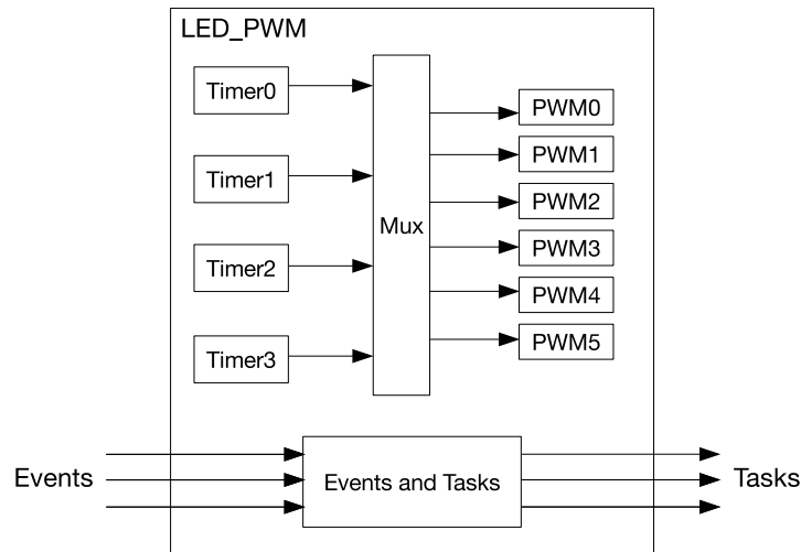
Figure 35.3-1. LED PWM Architecture
