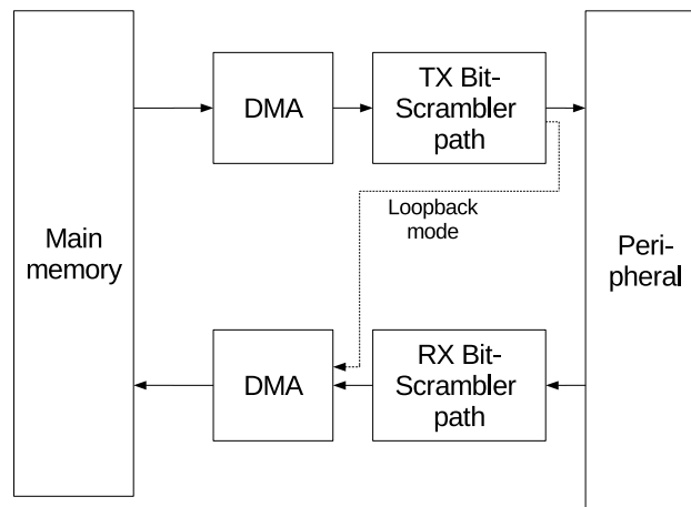
Figure 39.1-1. BitScrambler System Context Diagram
