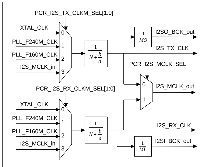
Figure 31.6-1. I2S Clock Generator
