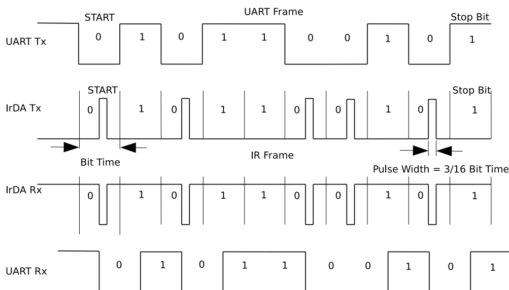
Figure 28.4-6. The Timing Diagram of Encoding and Decoding in SIR mode
