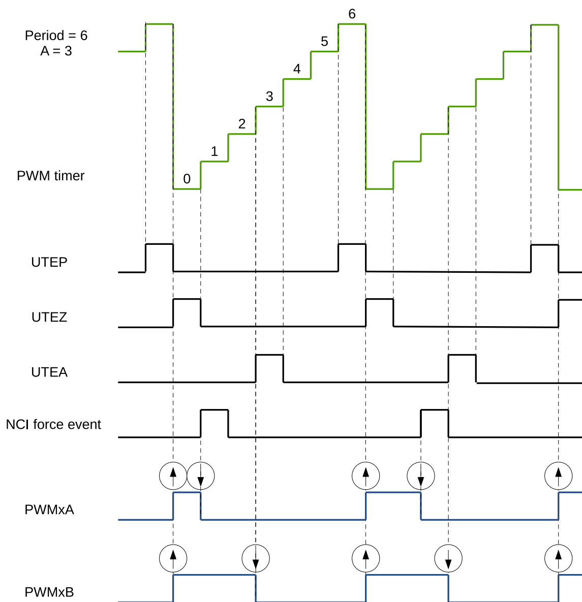
Figure 36.3-19. Example of an NCI Software-Force Event on PWMxA
