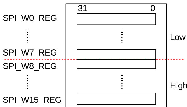
Figure 29.5-1. Data Buffer Used in CPU-Controlled Transfer
