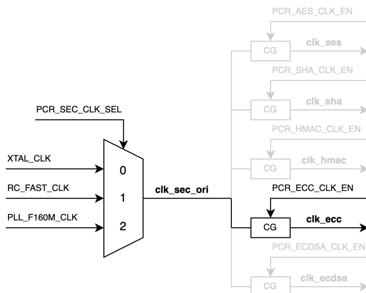
Figure 20.4-1. clk_ecc Diagram
