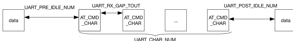
Figure 28.4-4. AT_CMD Character Structure
