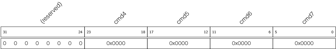
Figure 41.5-4. APB_SARADC_SAR_PATT_TAB2_REG Contains Patterns 4 - 7
