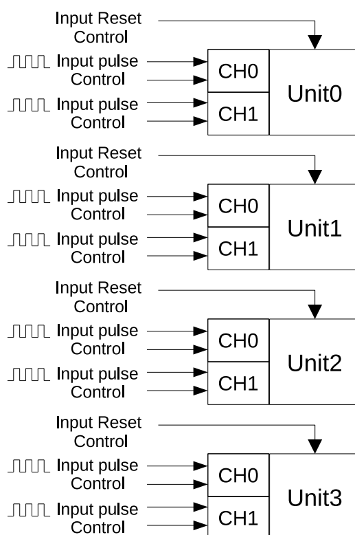
Figure 32.0-1. PCNT Block Diagram
