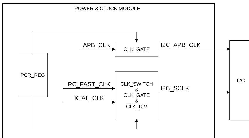
Figure 7.3-1. Clock Configuration Example
