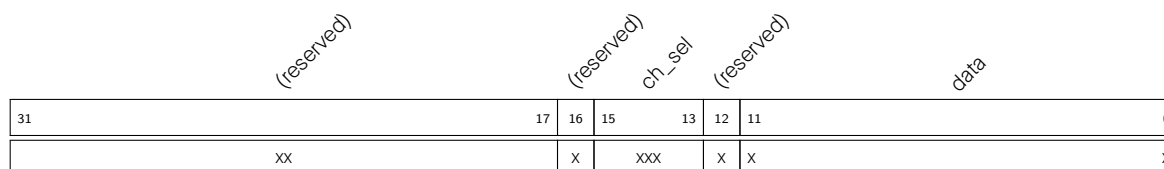
Figure 41.5-8. DMA Data Format
