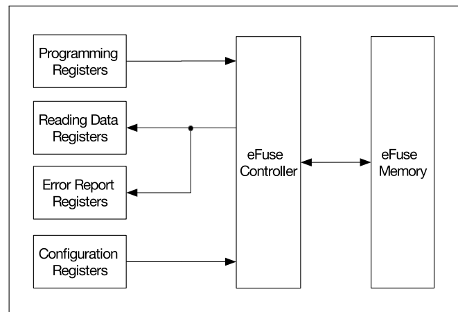
Figure 5.3-1. Data Flow in eFuse
