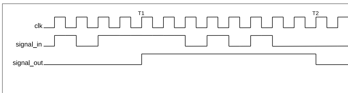
Figure 6.4-3. Glitch Filter Timing Example
