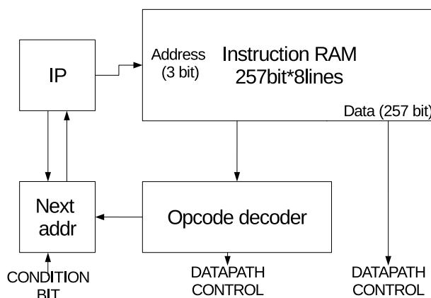
Figure 39.4-2. BitScrambler Control Path Diagram
