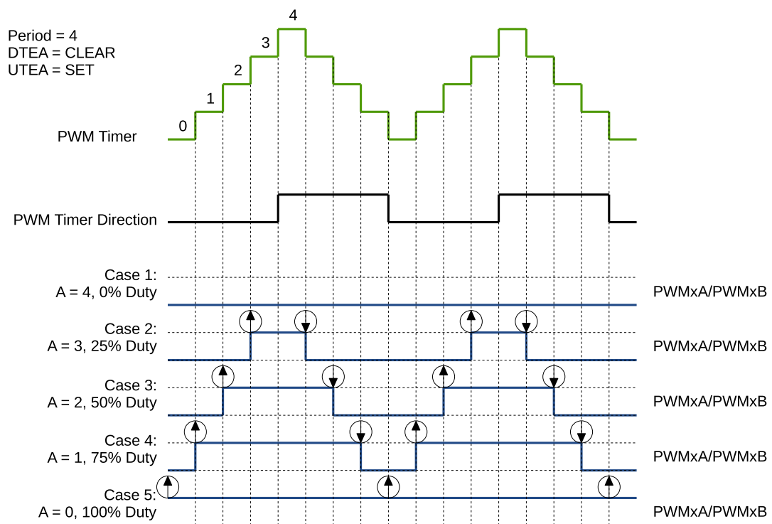
Figure 36.3-13. Symmetrical Waveform in Count-Up-Down Mode
