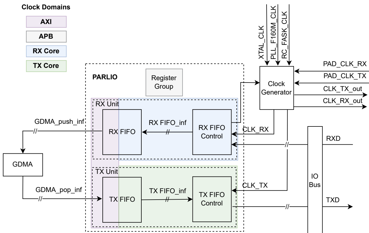
Figure 38.4-1. PARLIO Architecture
