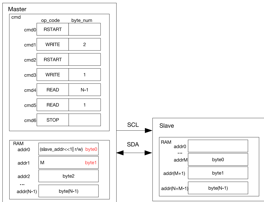
Figure 30.7-7. I2C master Reading N Bytes of Data from addrM of I2C slave with a 7-bit Address
