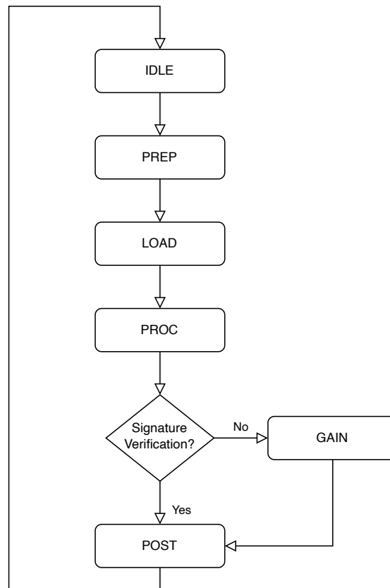
Figure 25.5-1. ECDSA Process
