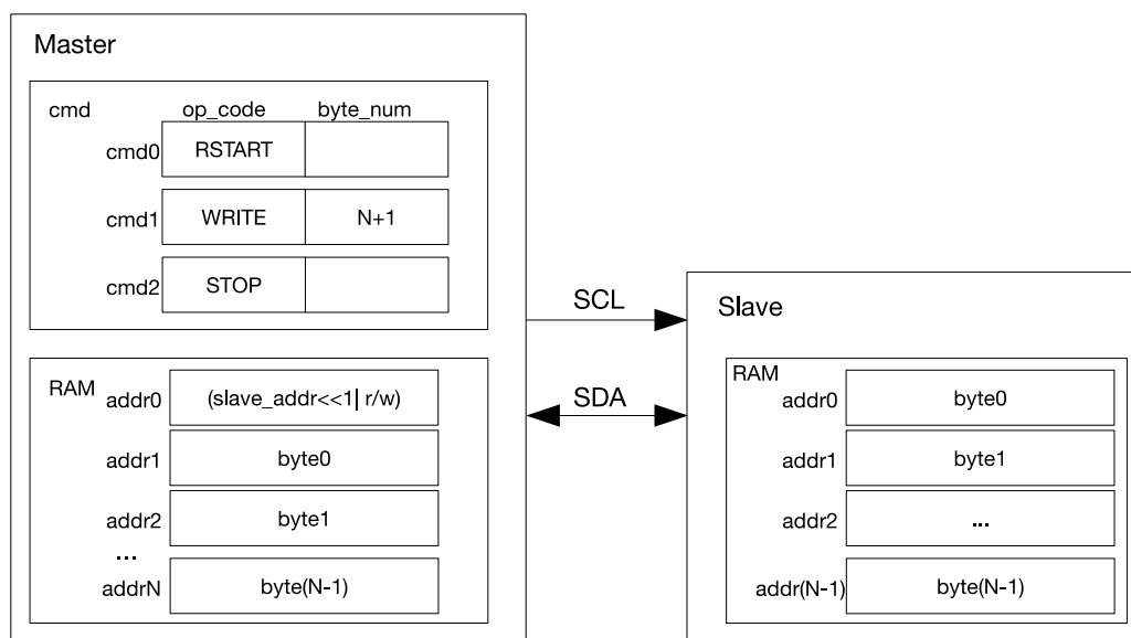
Figure 30.7-1. I2C master Writing to I2C slave with a 7-bit Address
