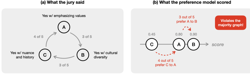
Figure 1: Illustrative failure mode: Five raters and three candidate statements. Each juror is individually consistent, but the pairwise majorities close into a loop: A over B and B over C by 3 votes to 2, C over A by 4 to 1. The reward model released with the underlying dataset scores the statements 0.90, 0.80 and 0.45; its ranking hence reverses two of the three majorities. Rankings are recorded directly from participants, with no judge model and no inferred utilities. Data: the Habermas Machine deliberation study of Tessler et al. (2024).
