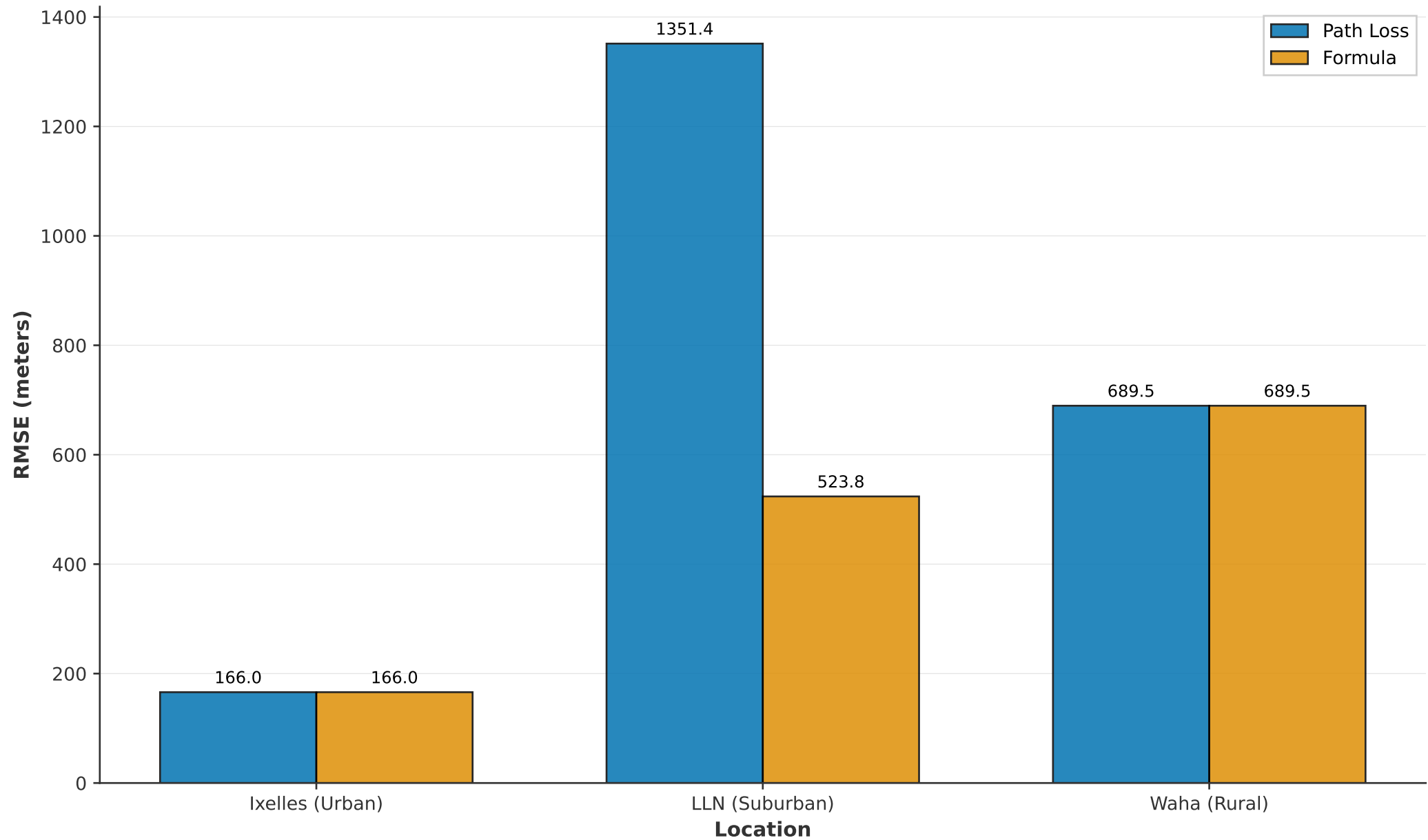
Trilateration Accuracy: Path Loss vs Formula
