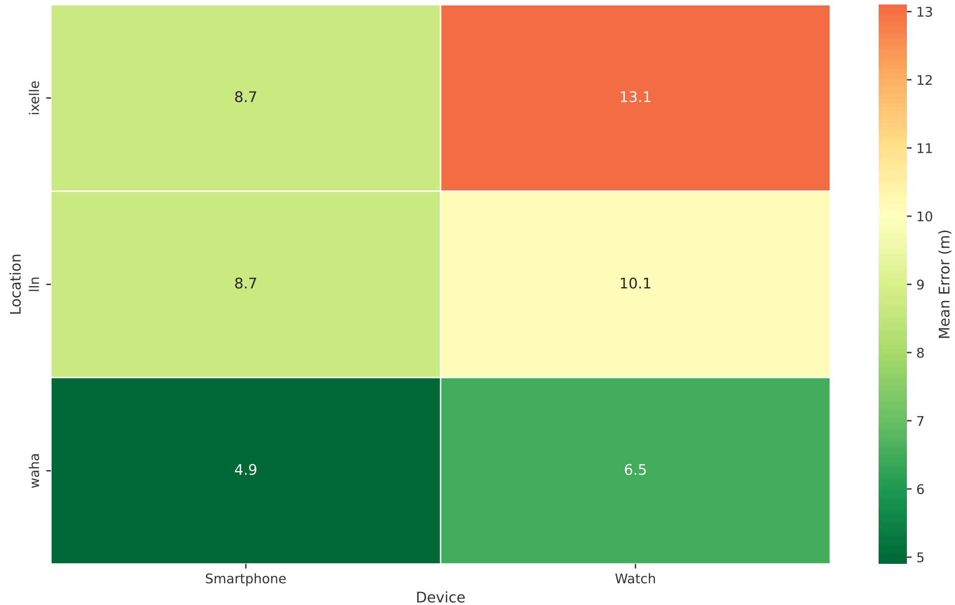
Figure 6: Mean GPS Error Heatmap (Location × Device)
