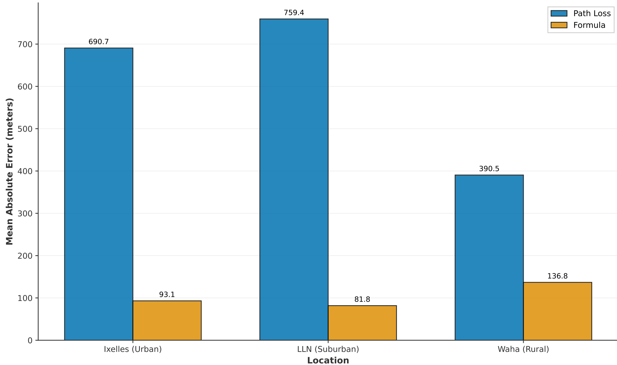
Distance Estimation Accuracy: Path Loss vs Formula
