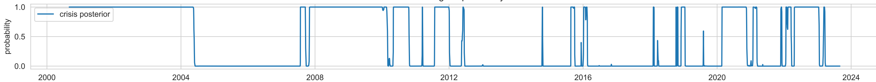
Crisis regime probability
