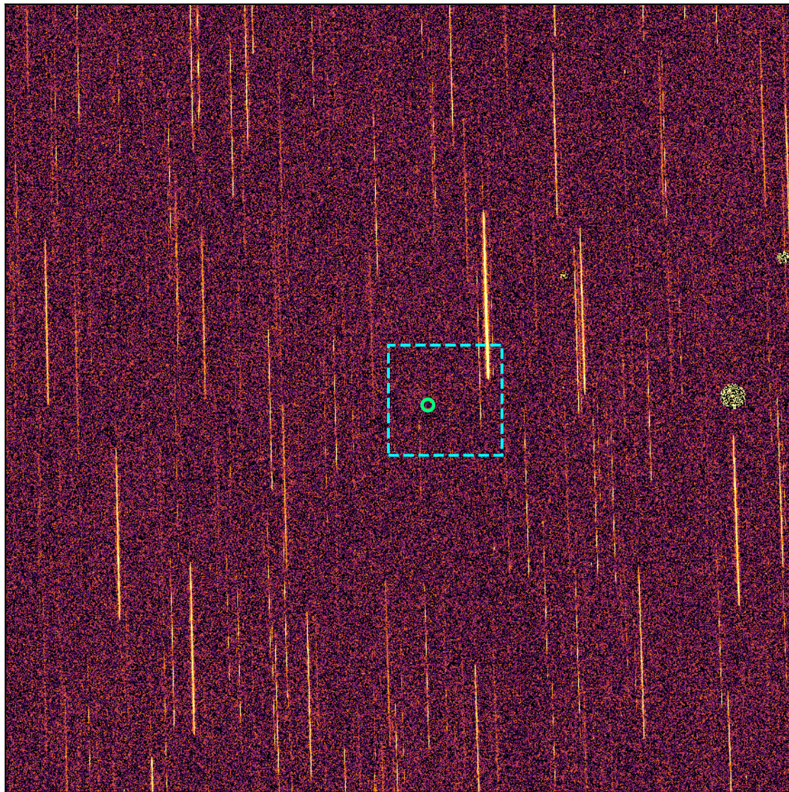
Roman WFI simulation — same sky, three views Grism (L2, SCA05) same 1' field dispersed (box)
