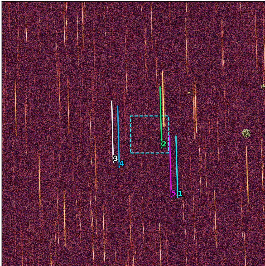
Grism (L2, SCA05) full SCA, 7.5' / 0.11" px
