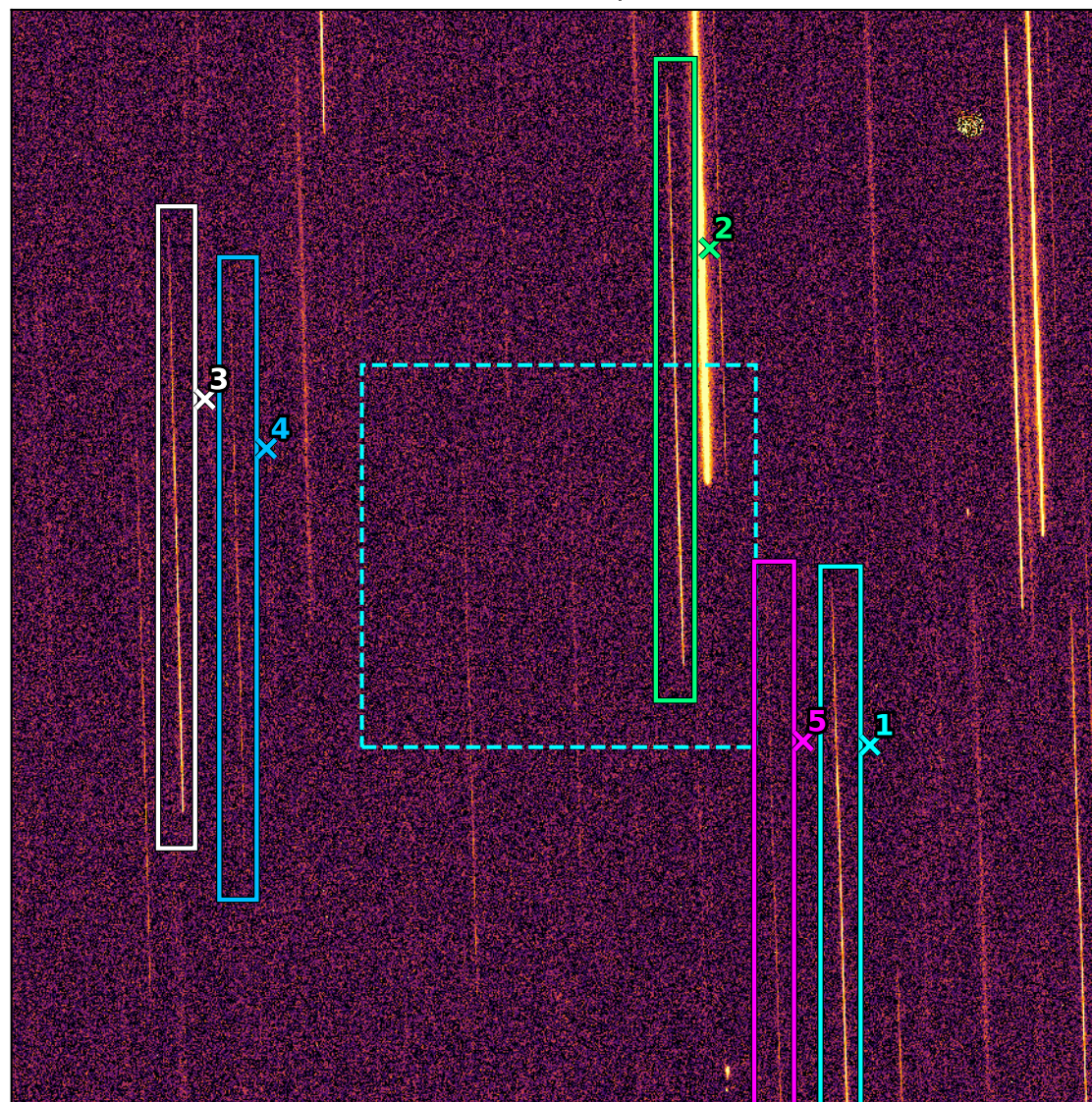
Roman WFI simulation — same sky, three views Grism (L2, SCA05) 3' / 0.11" px
