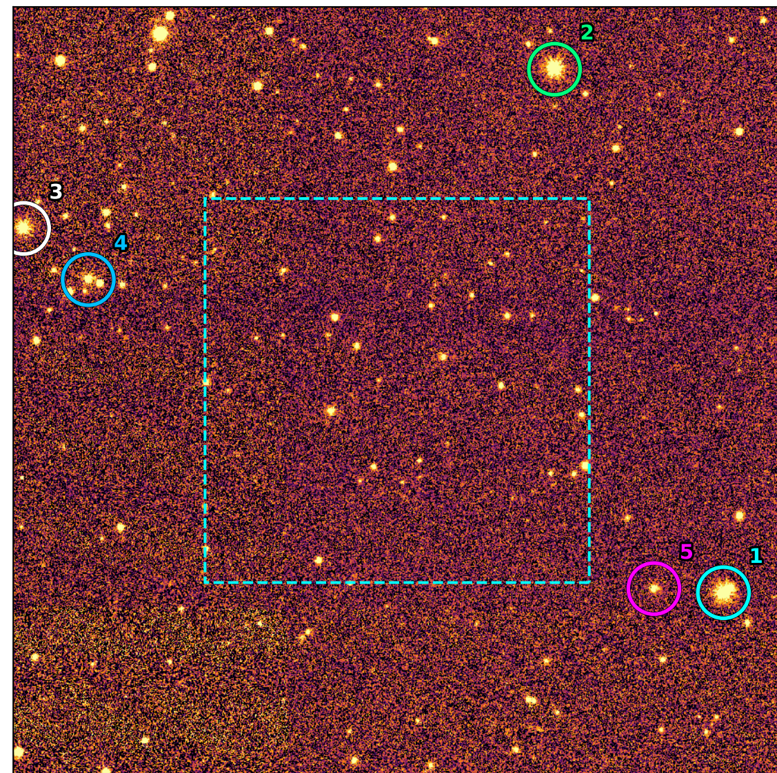
Imaging F158 (L3 coadd) 2' @ RA=10.183, Dec=-0.184
