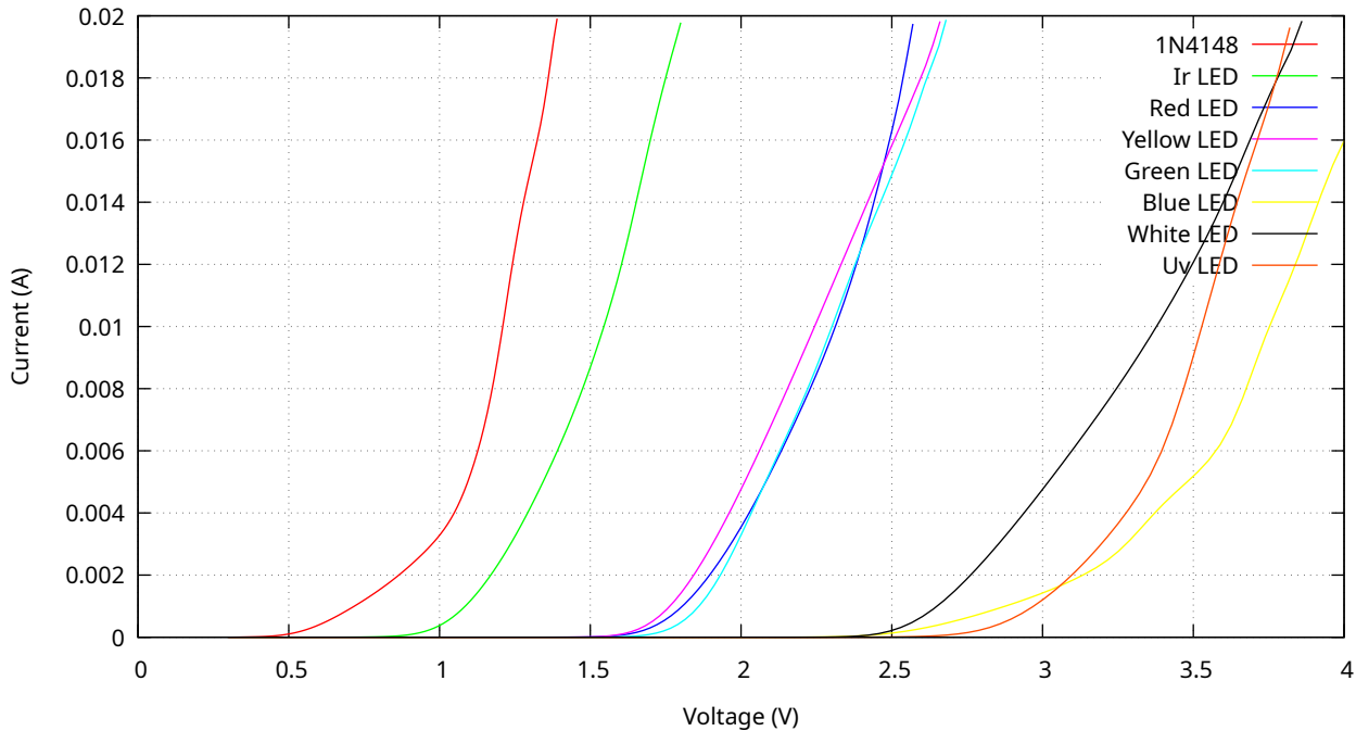
LED/Diode Characteristics
