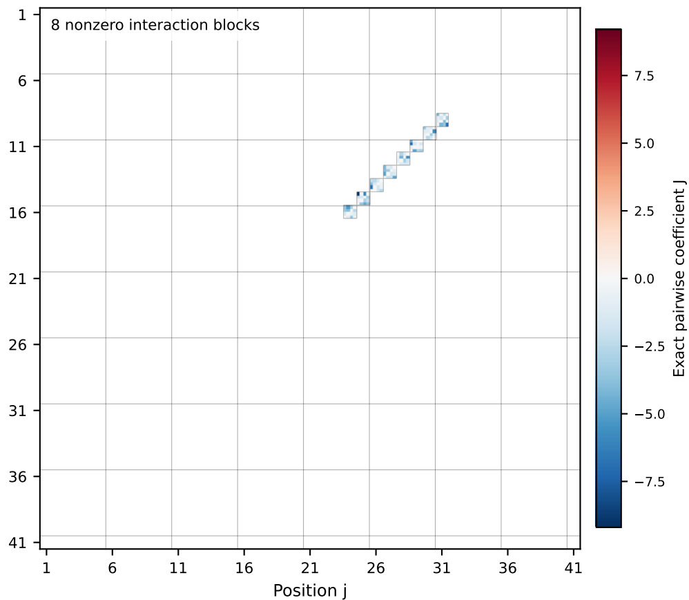
Pairwise matrix
