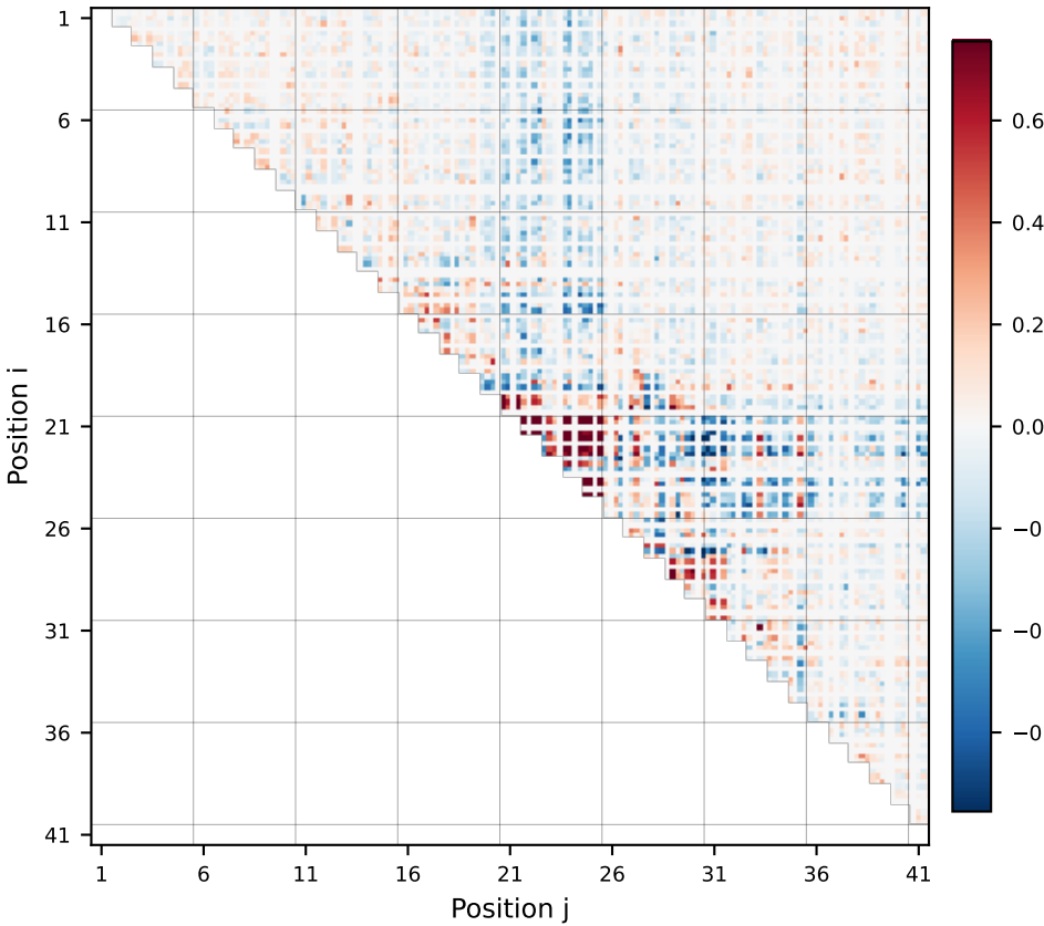
Pairwise matrix
