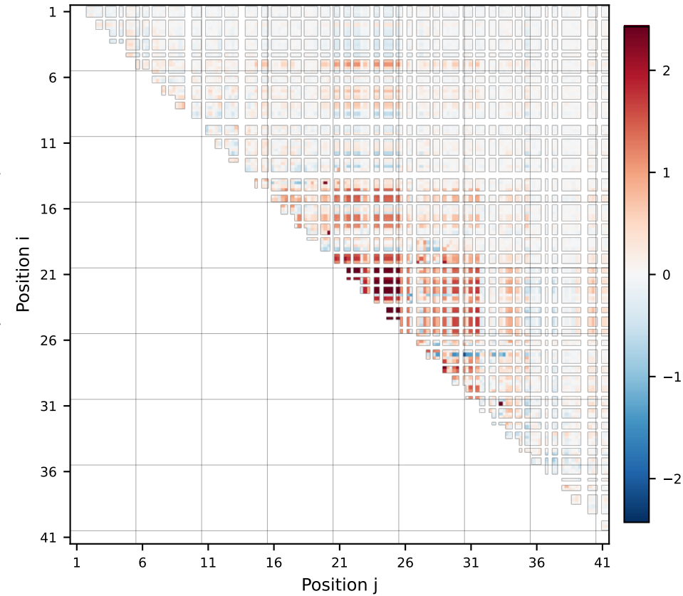
Activity epistasis
