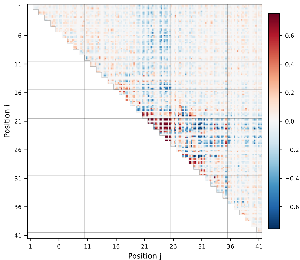
Pairwise matrix
