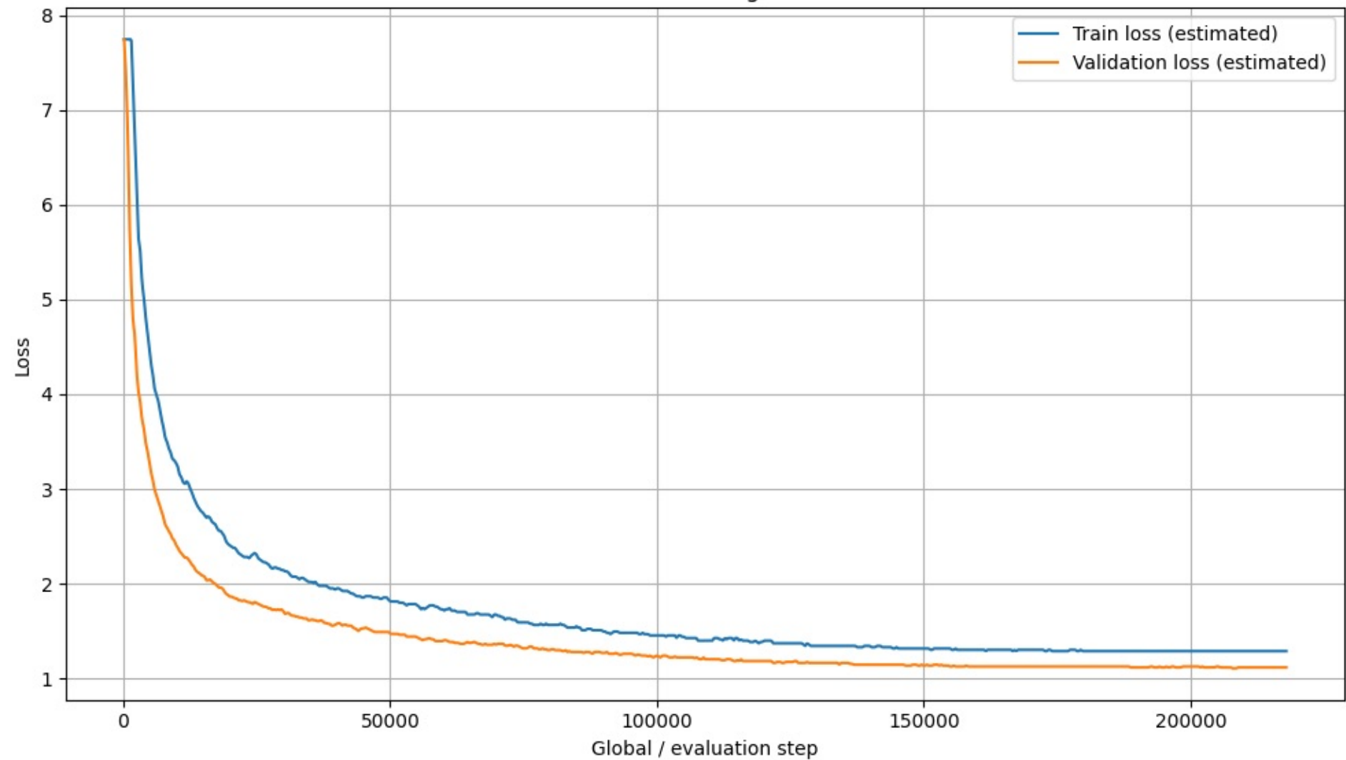
Estimated GPT-OSS Training vs Validation Loss
