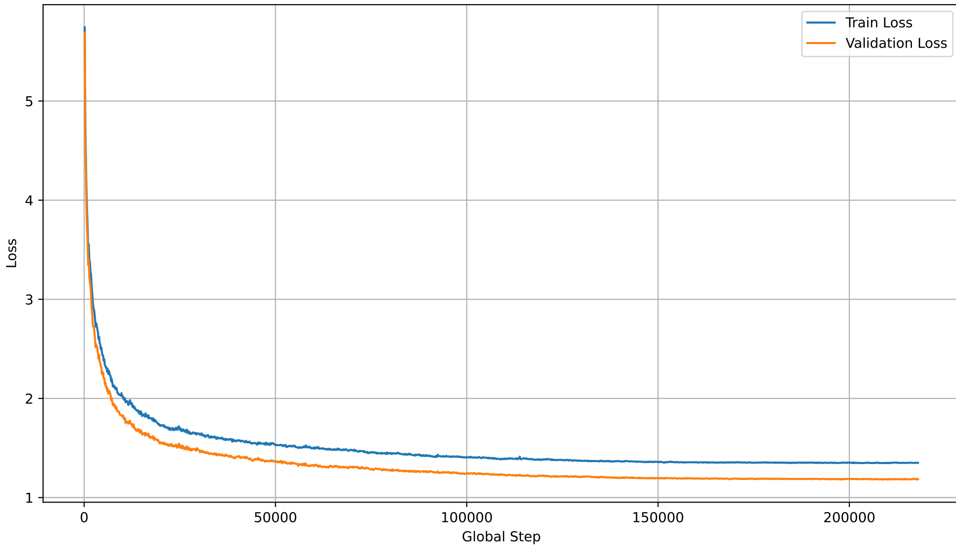
GPT-OSS Training vs Validation Loss
