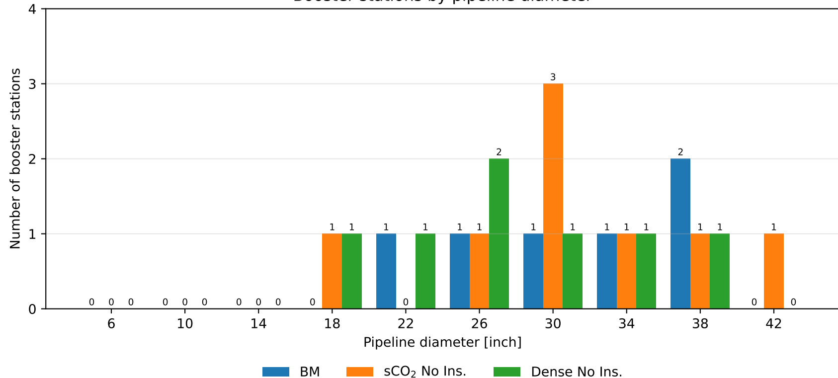
Booster stations by pipeline diameter
