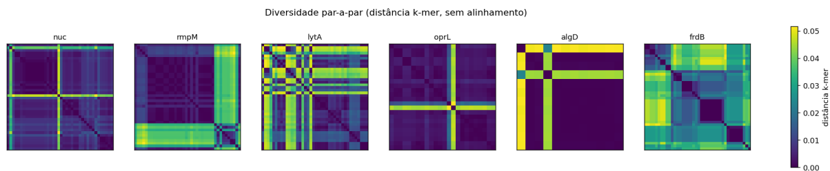
Figure 2: Pairwise 4-mer distance heatmaps per gene (alignment-free). Each cell is the 4-mer distance between two retrieved sequences of the gene.
