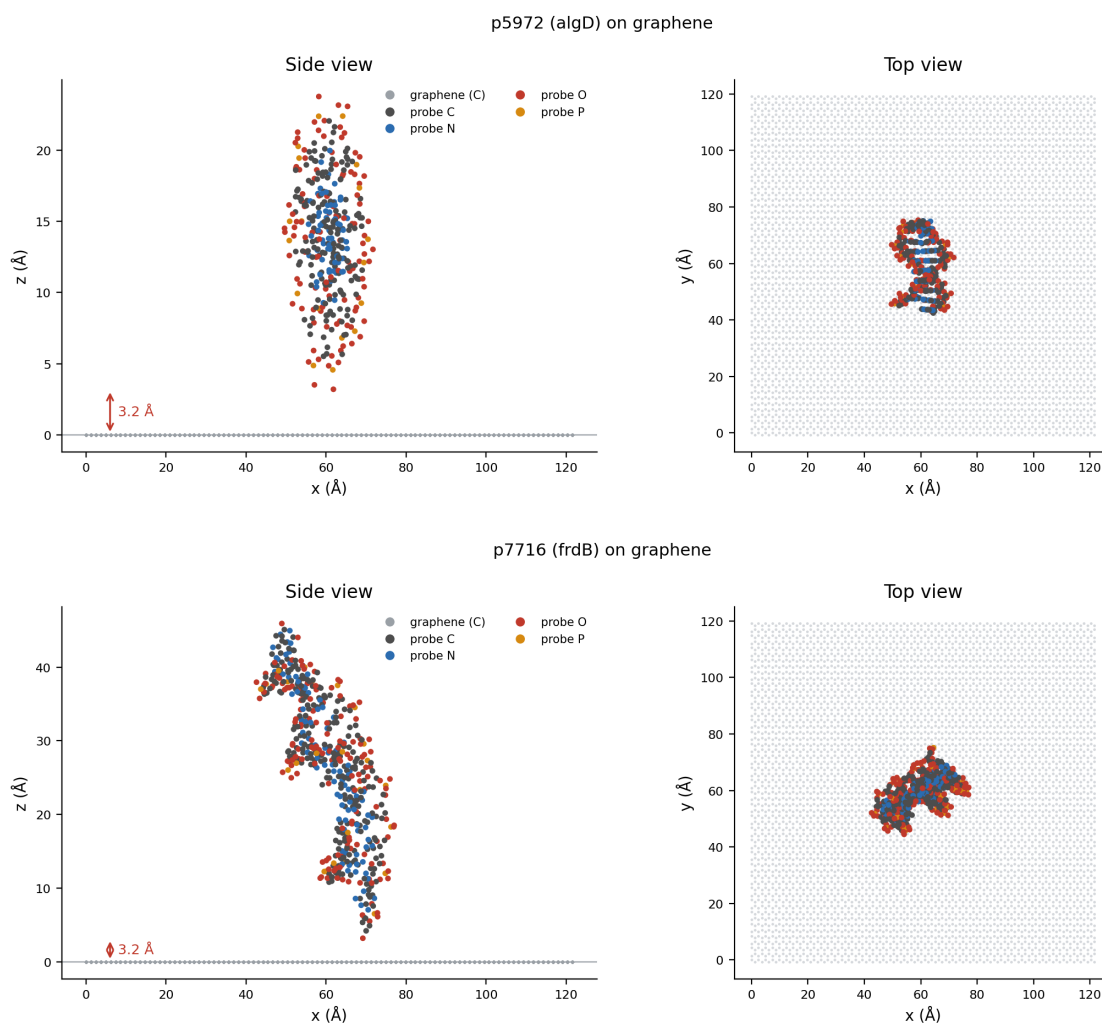
Figure 4: Assembled probe-graphene models for p5972 ( algD , top) and p7716 ( frdB , bottom), rendered from the model coordinates. Left: side view, with the graphene plane, the probe above it and the 3.2 Å separation indicated. Right: top view, showing the probe footprint within the 121.6 \times 119.8 Å sheet. Probe atoms are coloured by element; graphene carbons are grey.
