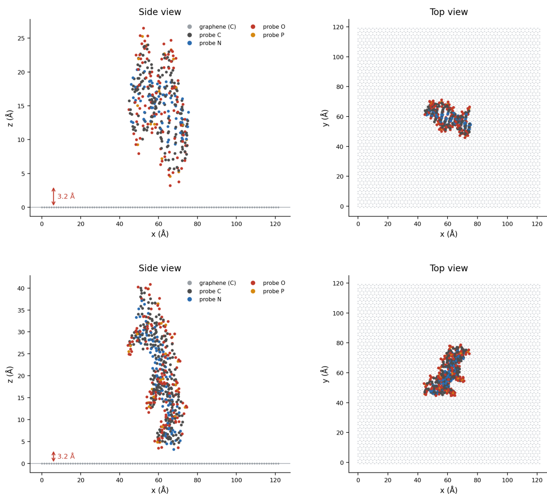
Figure 4: Assembled probe-graphene models for p5178 (algD) , top) and p6922 (frdB) , bottom), rendered from the model coordinates. Left: side view, with the graphene plane, the probe above it and the 3.2 Å separation indicated. Right: top view, showing the probe footprint within the 121.6 \times 119.8 Å sheet. Probe atoms are coloured by element; graphene carbons are grey.
