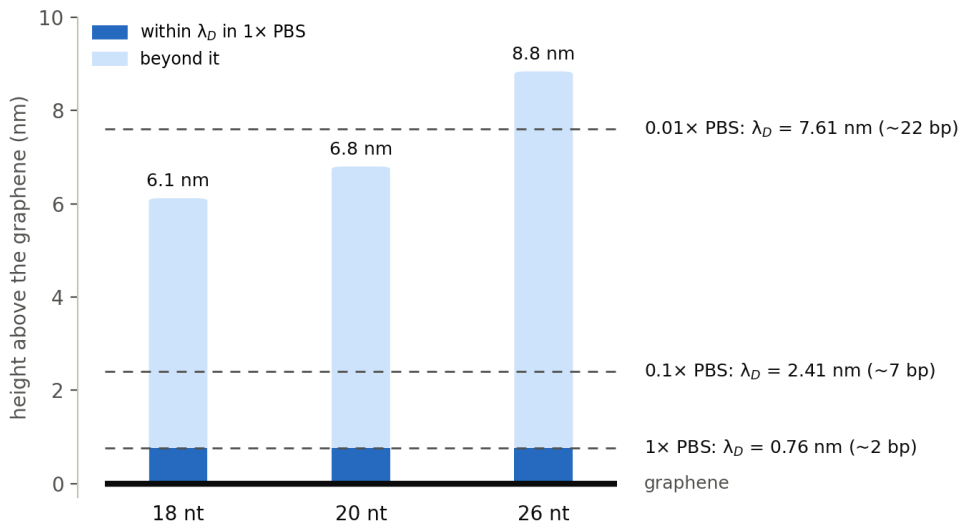
Figure 5: Length of a hybridised probe (B-form duplex, 0.34 nm per base pair (Watson and Crick, 1953)) for the shortest, median and longest probes selected (18, 20 and 26 nucleotides), compared on the same vertical scale with the Debye length of the three PBS dilutions (Purwidyantri et al., 2021). The dark segment is the part within \lambda_D in 1\times PBS. The geometry is the most favourable one: a duplex perpendicular to the surface and touching it, without a linker.
