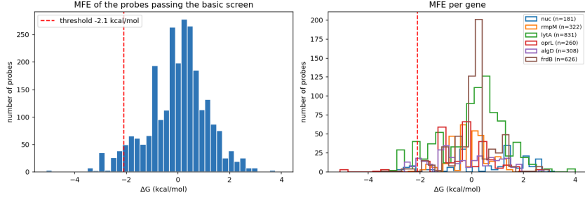
Figure 1: Distribution of the seqfold secondary-structure free energy ( \Delta G_{\text{MFE}} ) of the candidates that pass the basic screen in 1\times PBS, overall (left) and per gene (right), with the -2.1 kcal/mol threshold (fifth percentile).
