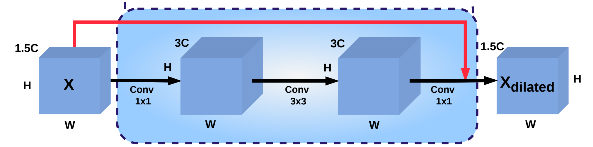
Dilated Bottleneck Block
