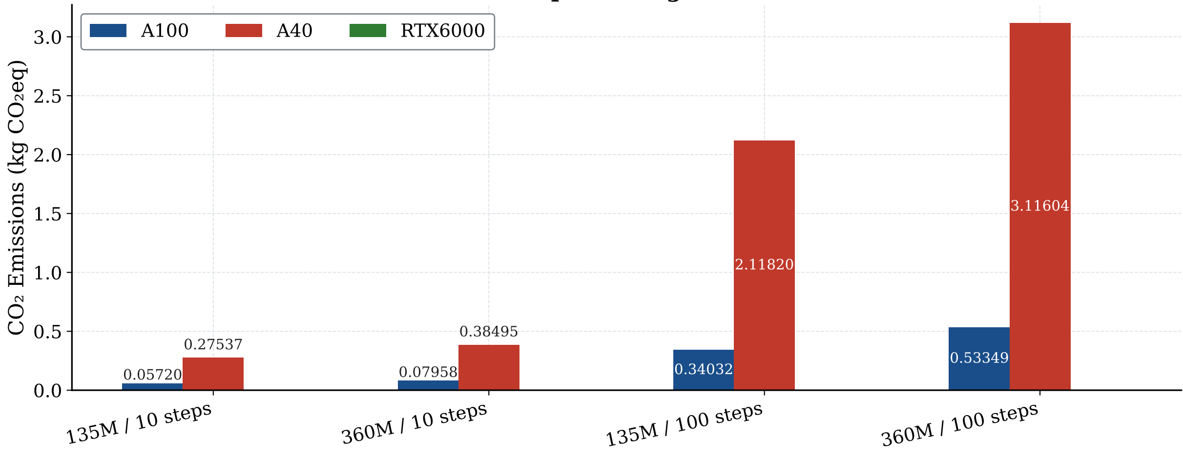
CO 2 Emissions per Configuration and GPU
