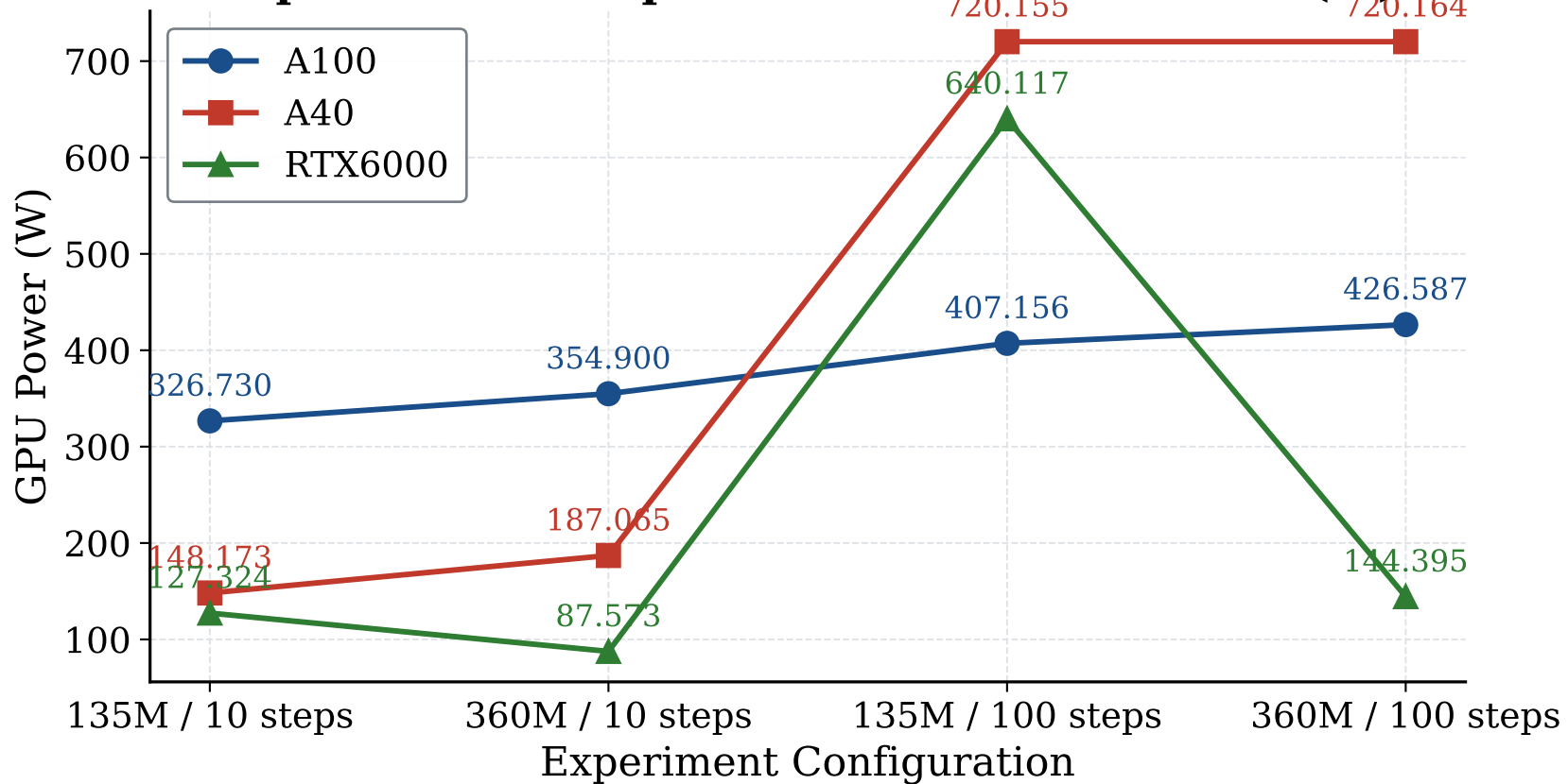
Experimental Response Values — GPU Power (W)
