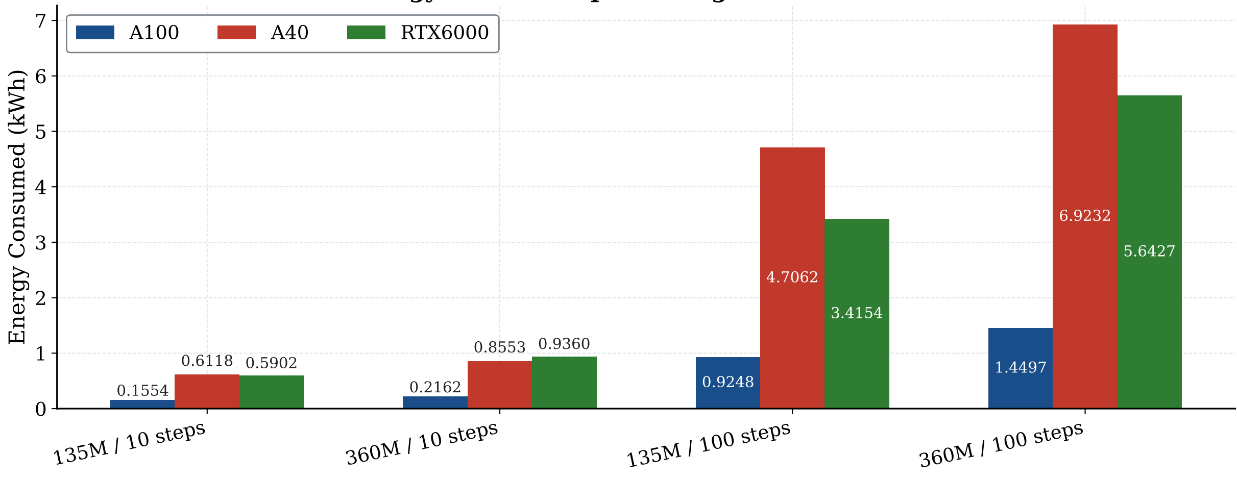
Energy Consumed per Configuration and GPU
