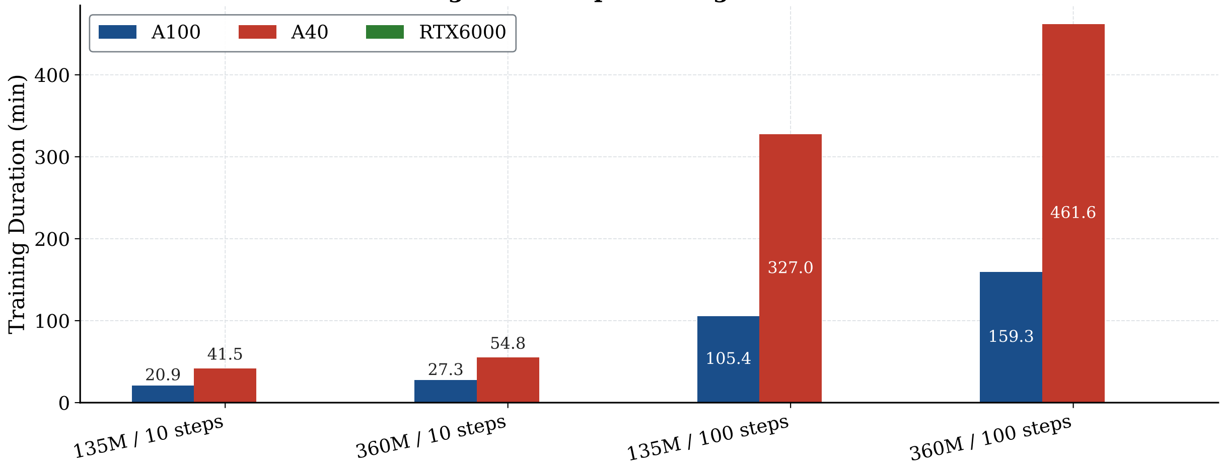
Training Duration per Configuration and GPU
