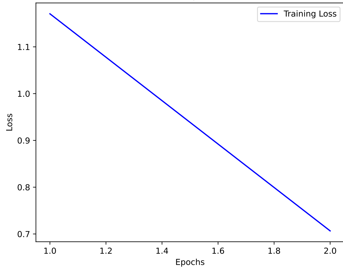
Training Loss
