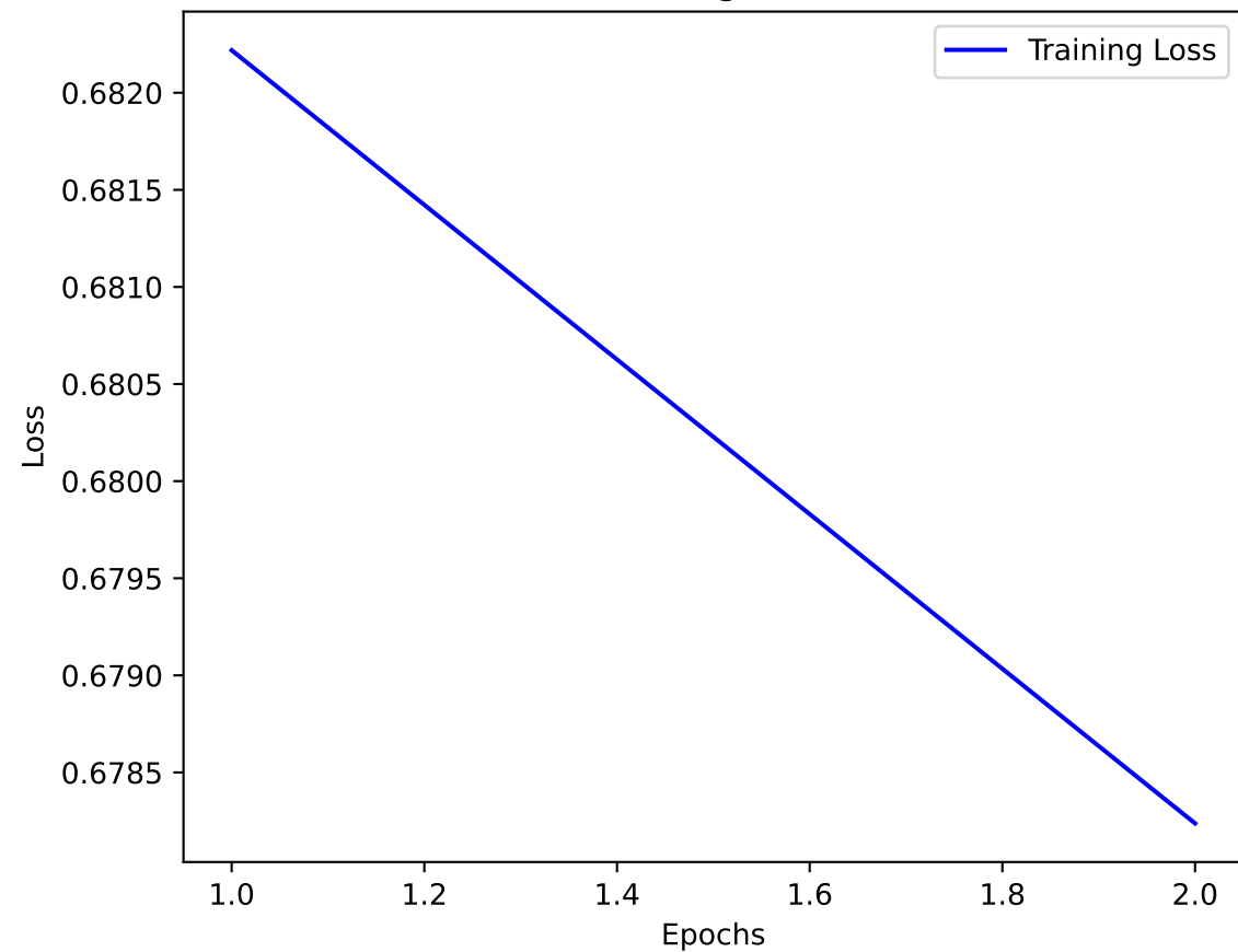
Training Loss
