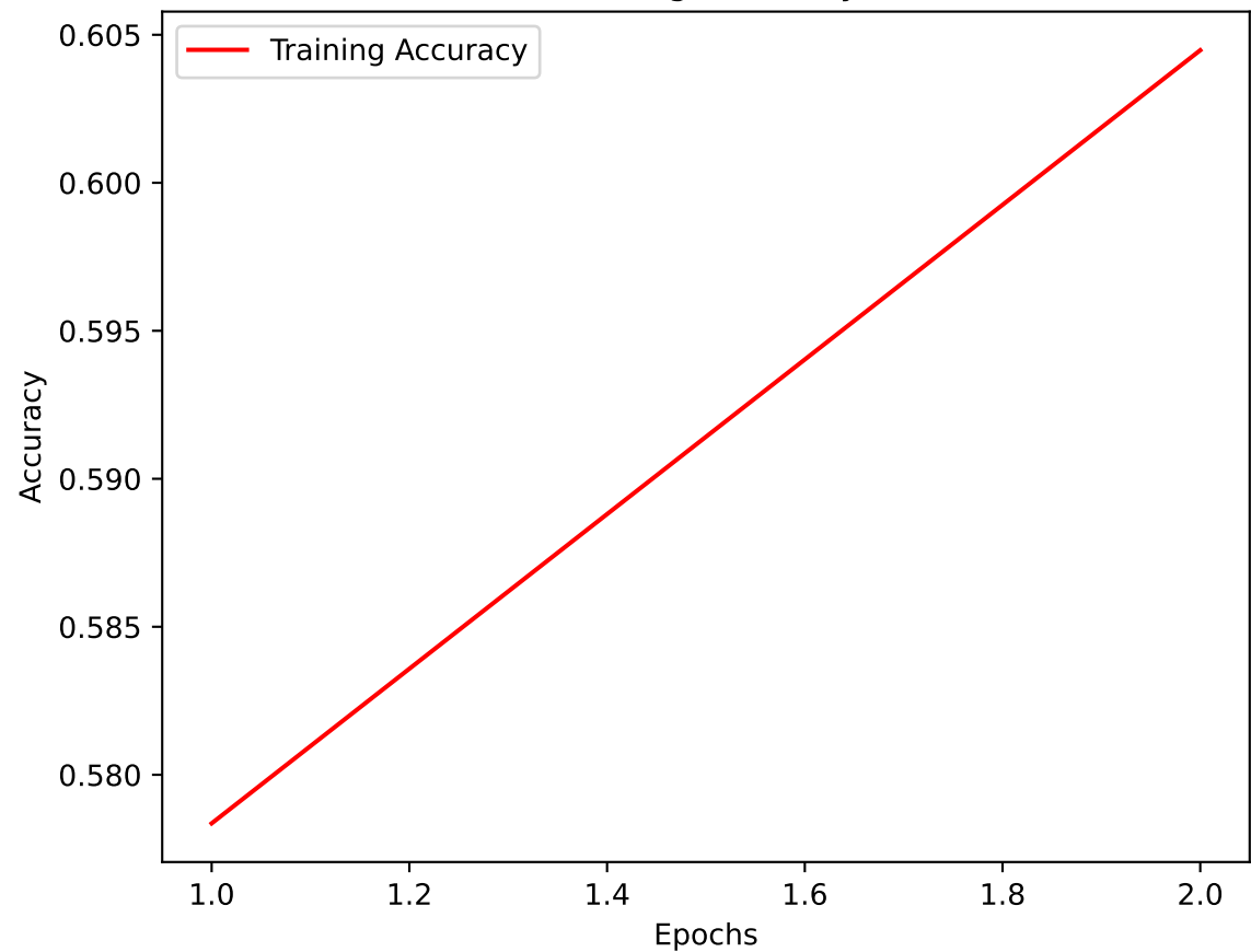
Training Accuracy
