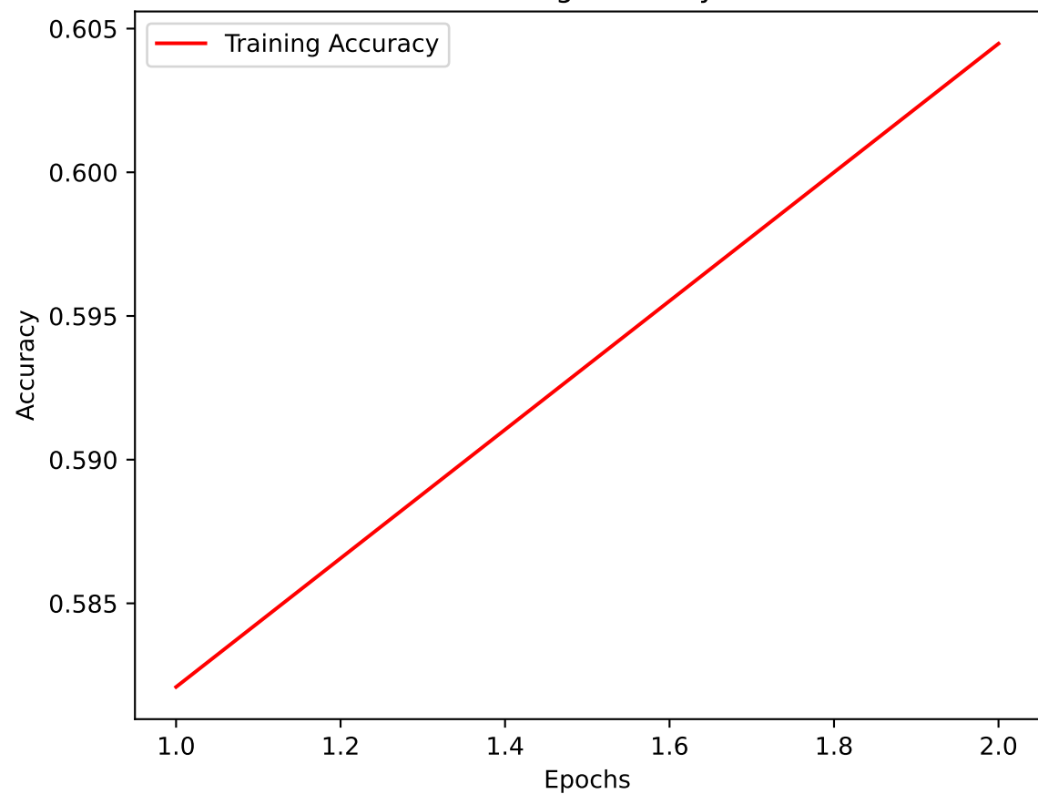
Training Accuracy
