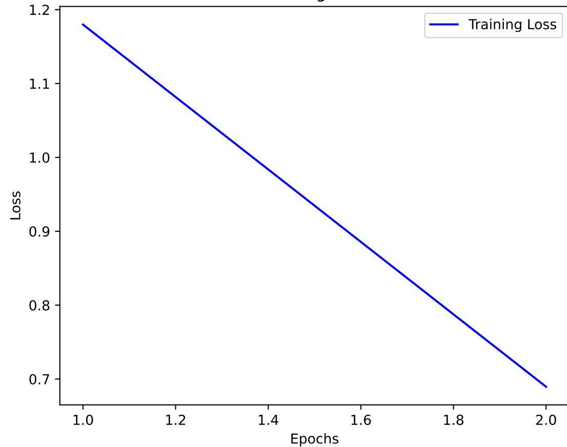
Training Loss
