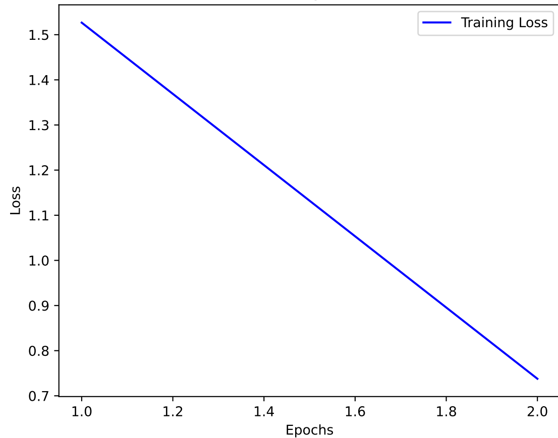
Training Loss
