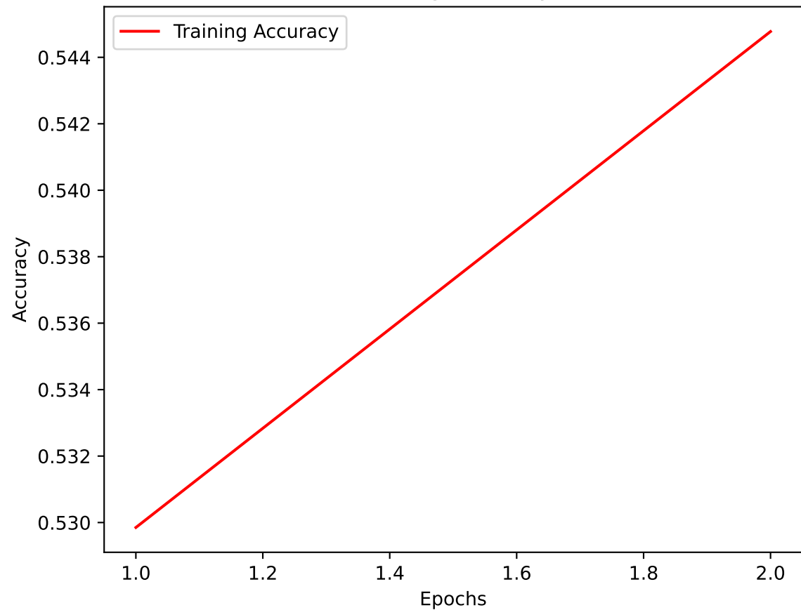
Training Accuracy
