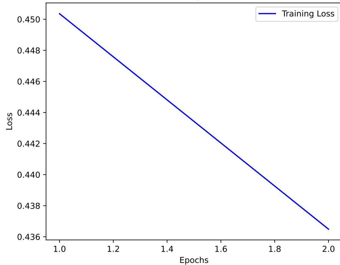
Training Loss
