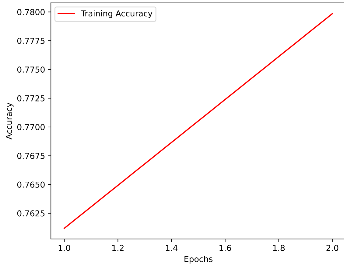
Training Accuracy
