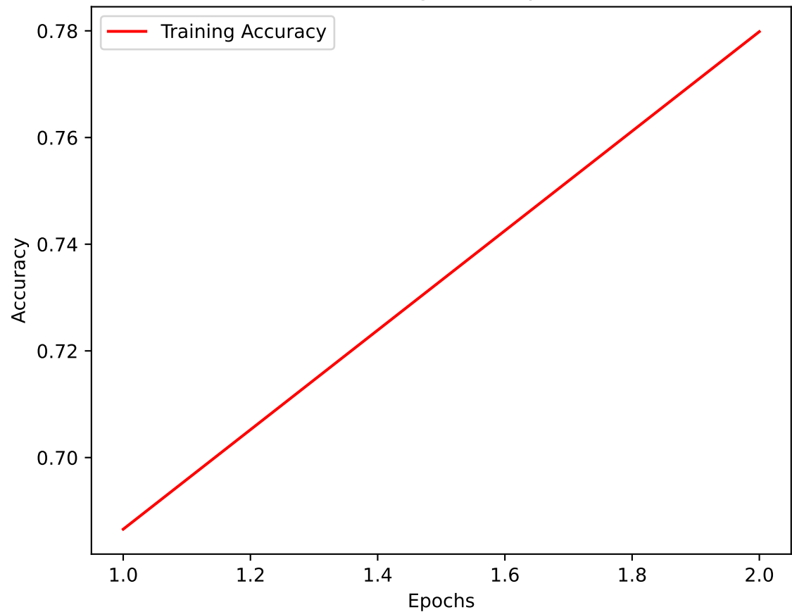
Training Accuracy
