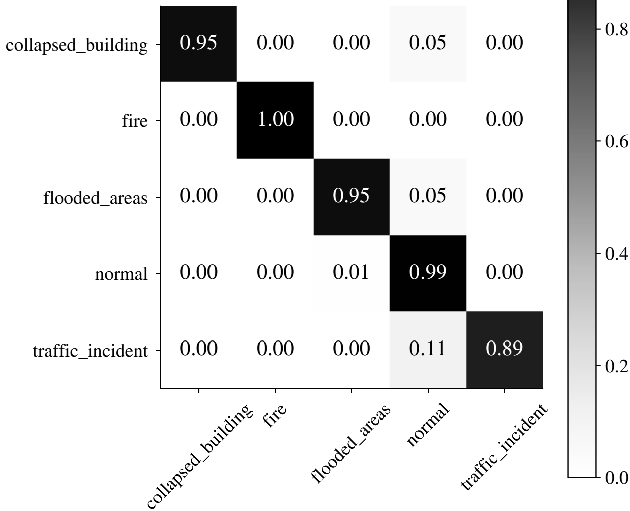
Predicted label
