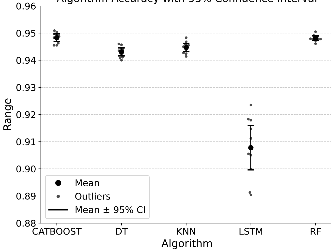
Algorithm Accuracy with 95% Confidence Interval
