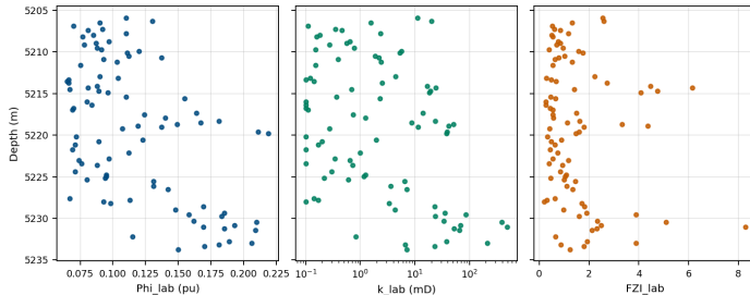
Well 861 MOGNO -- lab properties (5205.91--5233.72 m, n=87)
