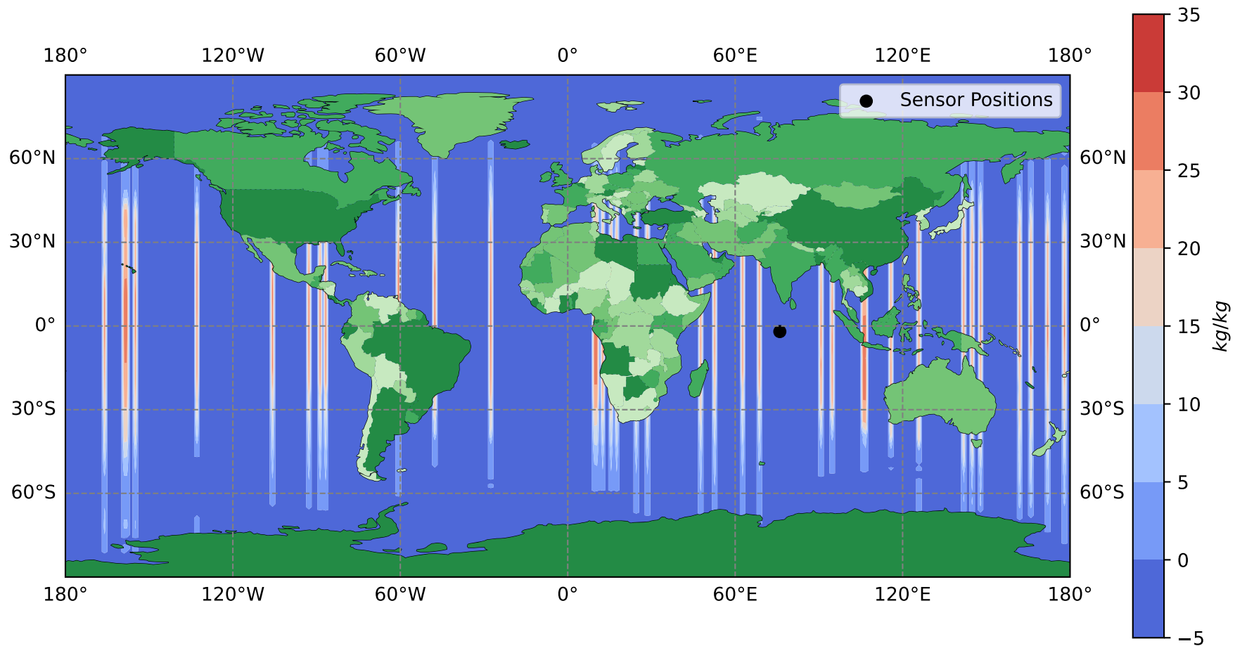
QMAX Subsampled - Last Snapshot
