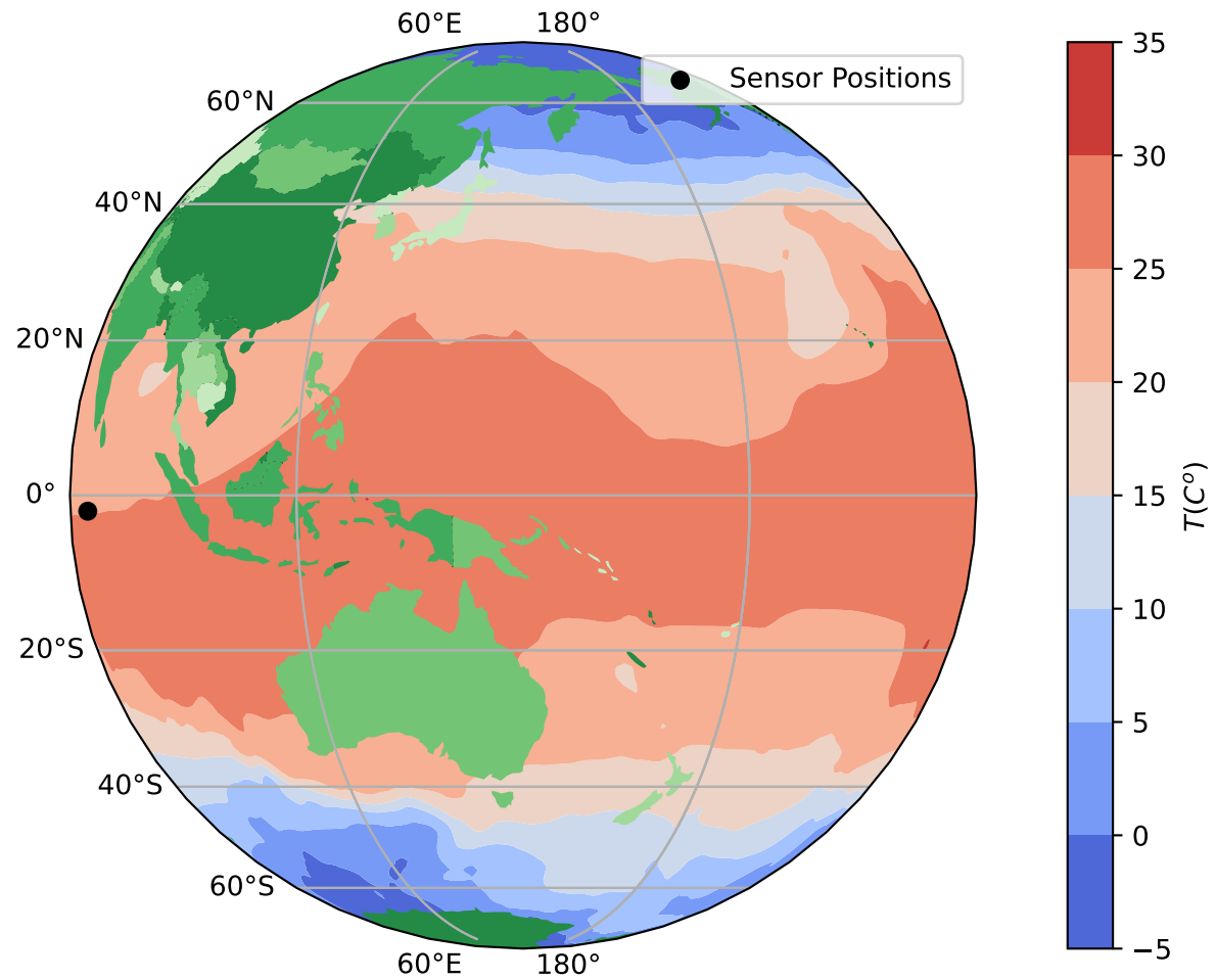
SST Original - Last Snapshot
