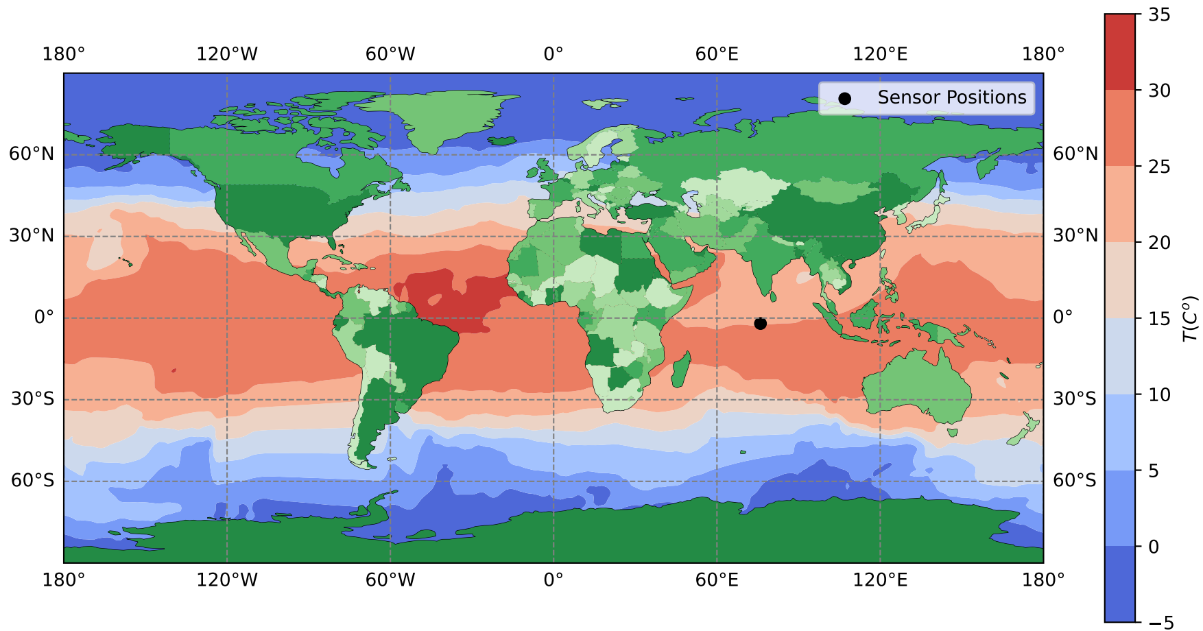
SST Original - Last Snapshot
