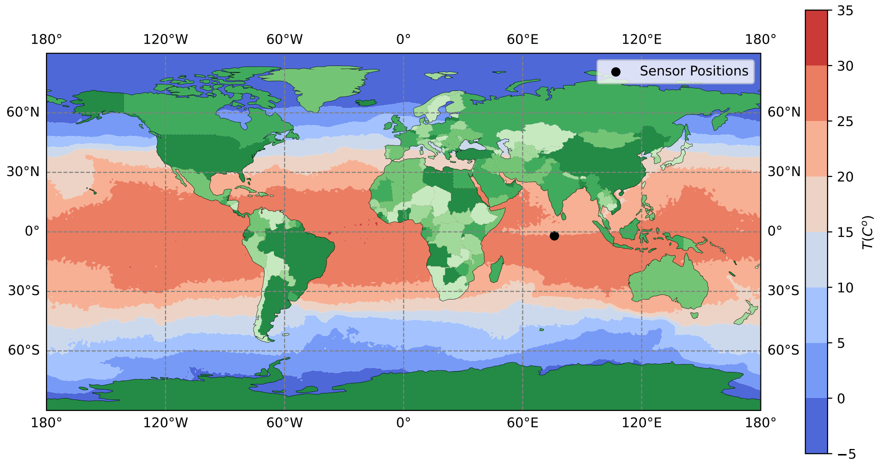
SST Reconstructed - Last Snapshot
