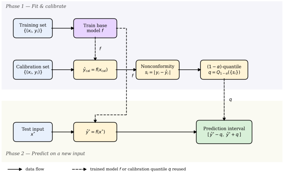
Figure 3: Inductive Conformal Prediction pipeline
