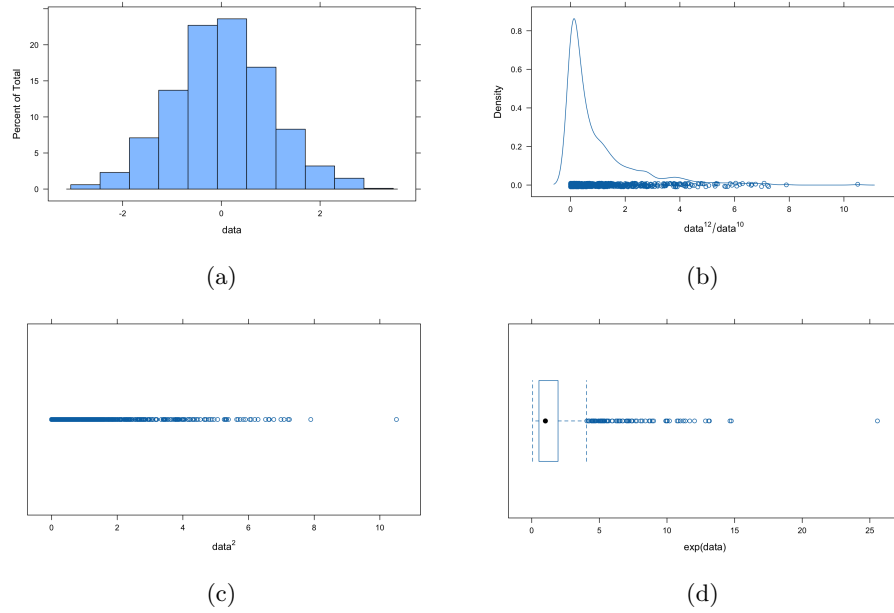
Figure 1: Different plots of the same data, sometimes transformed. No particular objective other than it being an exercise
