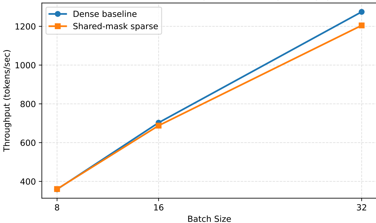
Dense vs. Shared-Mask Sparse Decoding Throughput
