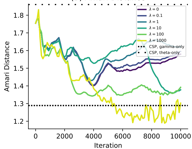
(B) Amari Distance
