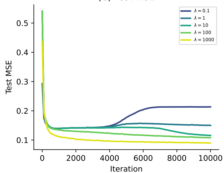
(C) Test MSE
