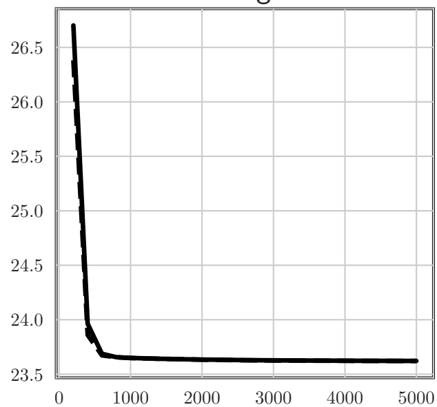
Unmixing Loss
