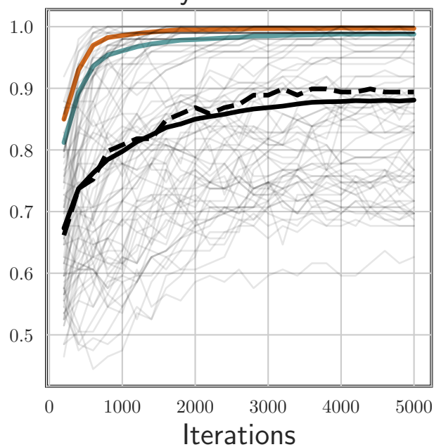
Accuracy: Stim. Protocol
