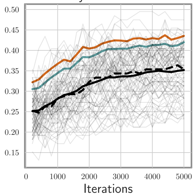
Accuracy: Reach Direction
