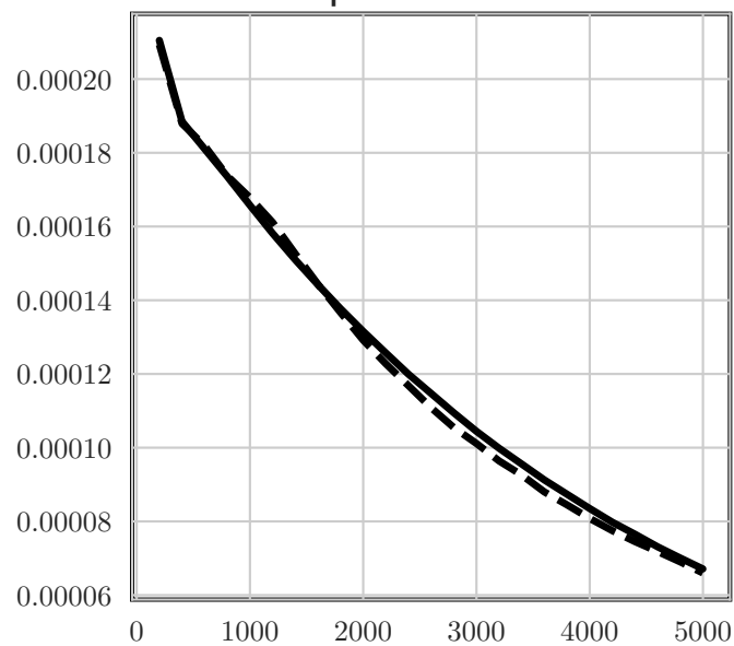
Supervised Loss
