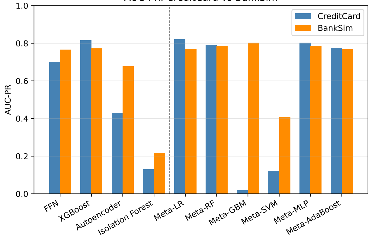
AUC-PR: CreditCard vs BankSim
