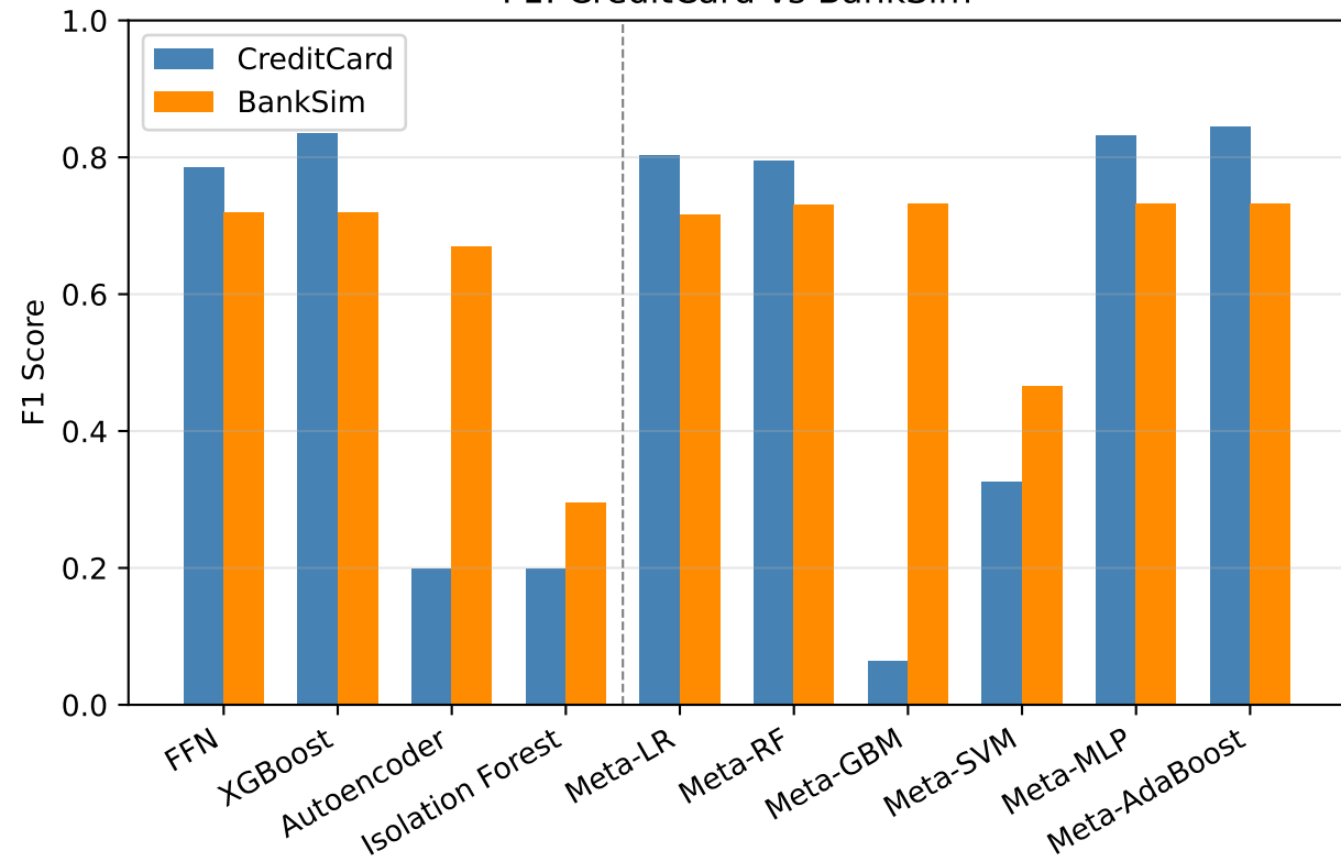
F1: CreditCard vs BankSim
