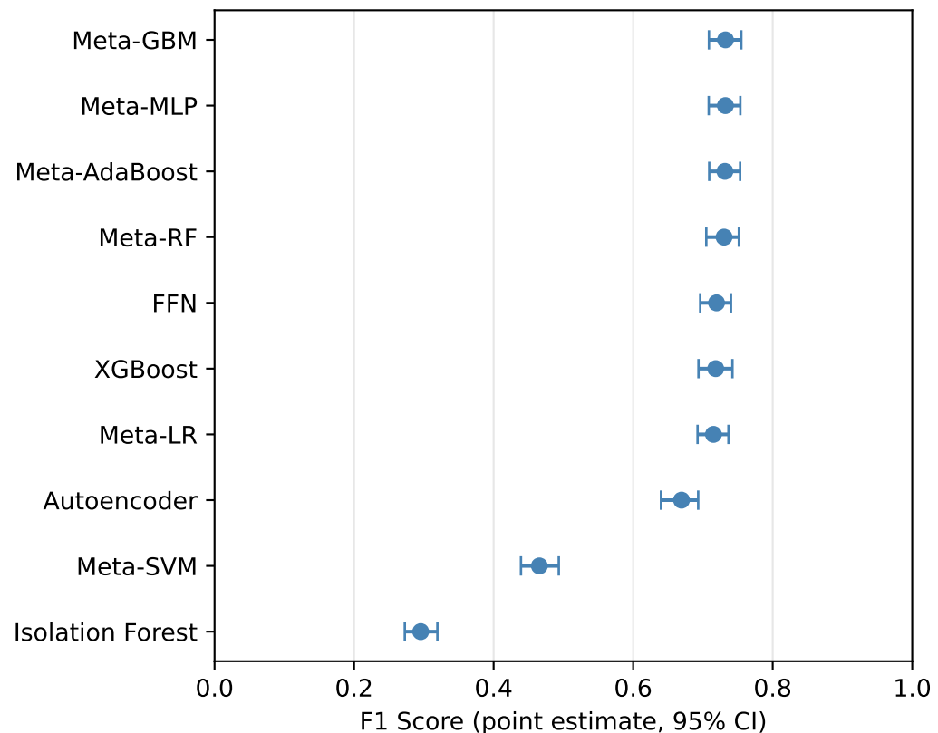
BankSim
