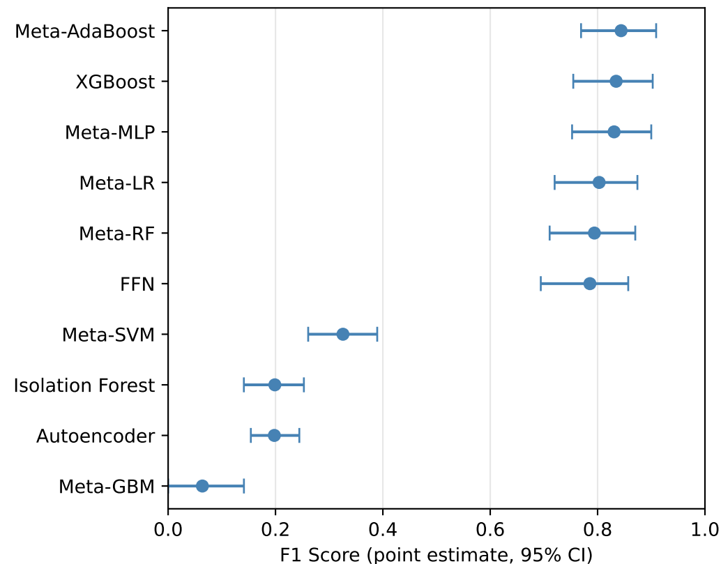
CreditCard
