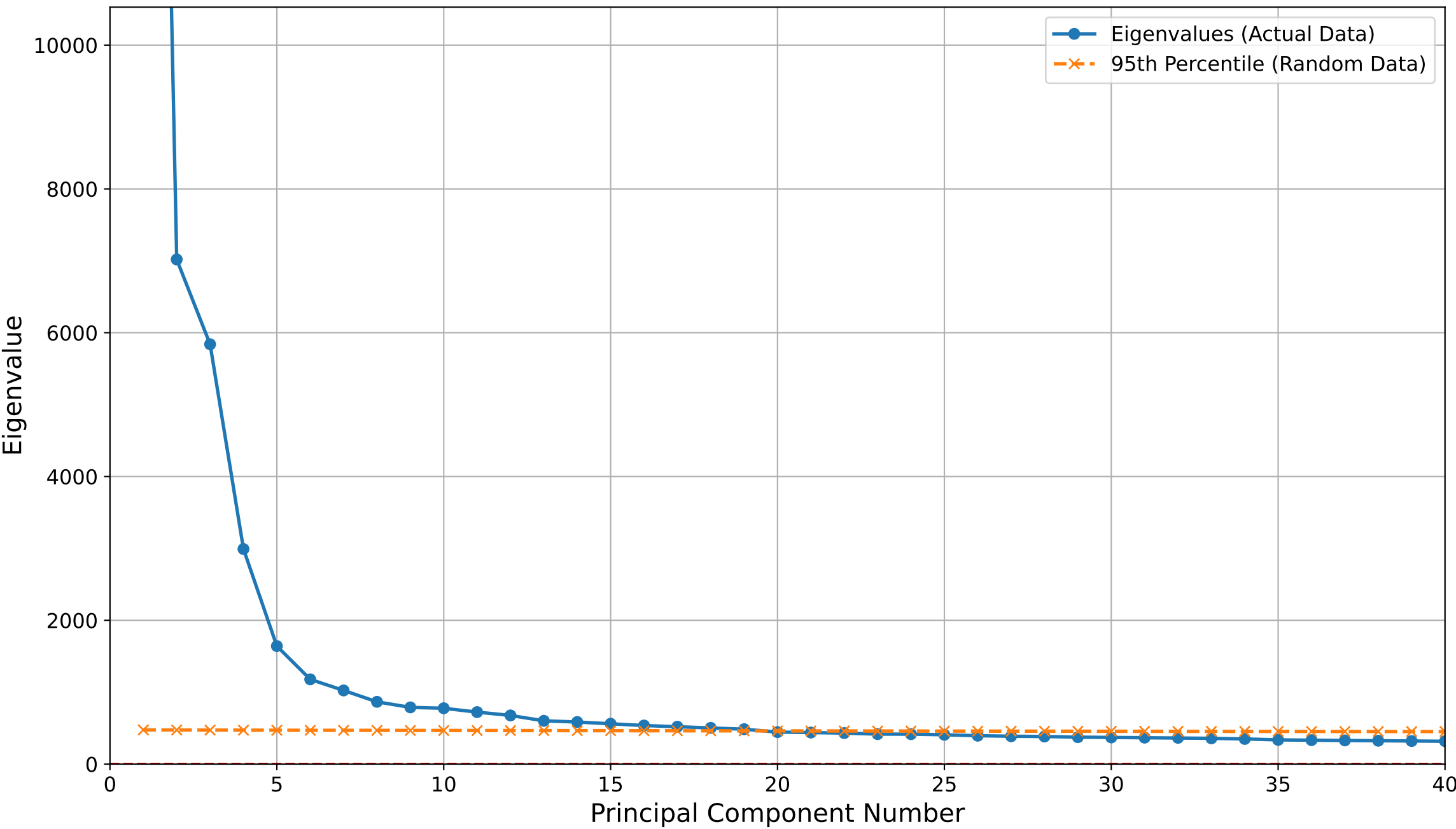
Corrected Scree Plot (on Normalized Data)
