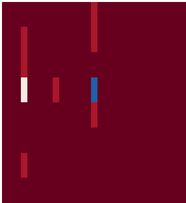
SciCode ( \hat{P} )
