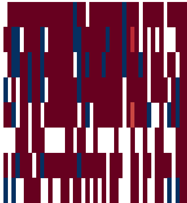
CoreBench-Hard ( \hat{P} )
