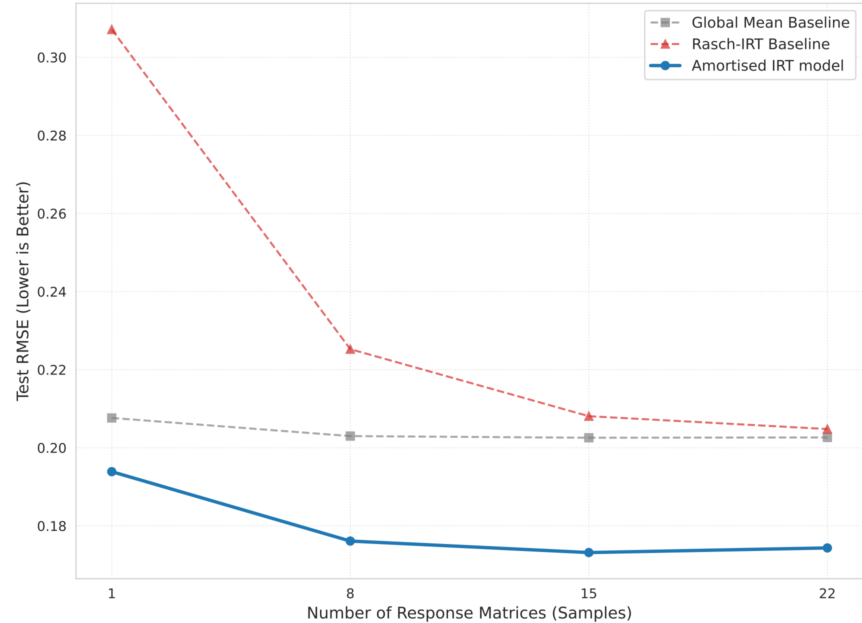
RMSE Convergence Analysis
