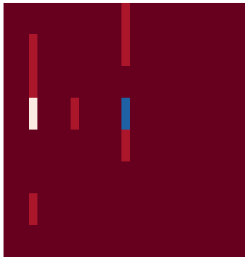
SciCode ( \hat{P} )
