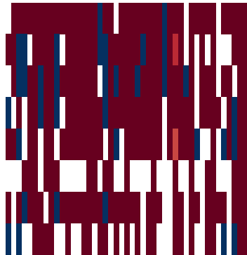
CoreBench-Hard ( \hat{P} )
