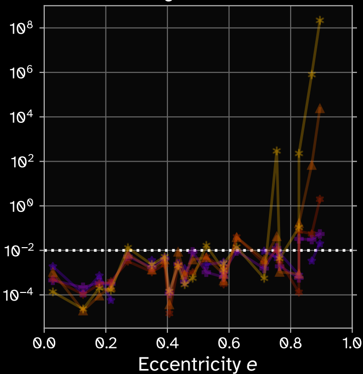
Integrator: RK12
