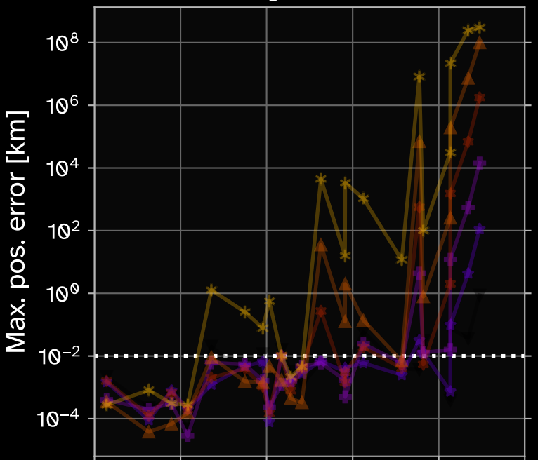
Integrator: RK10
